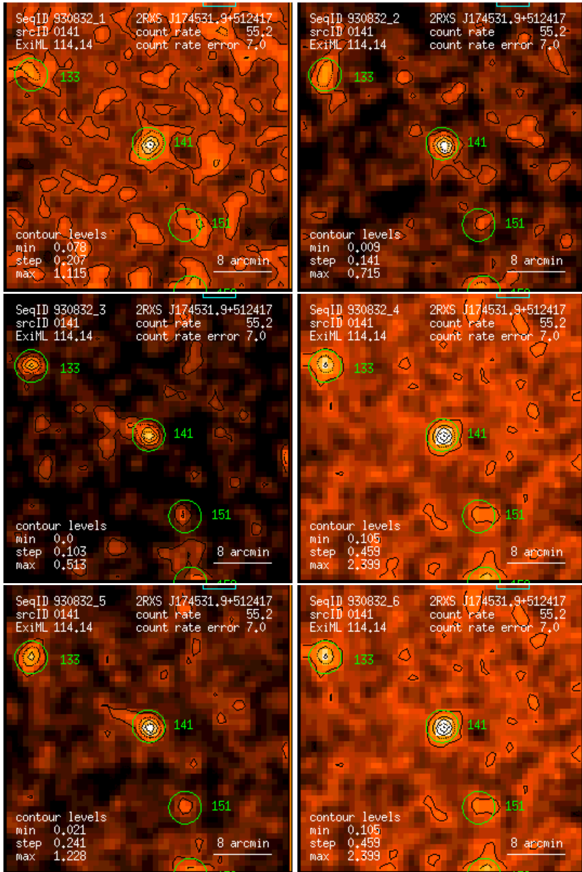
Figure 141: RASS 930832: detection 0141: band rate images, Gaussian filter: (1) PSPC channels 11 – 41, (2) 52 – 90, (3) 91 – 201, (4) 11 – 235, (5) 52 – 201, (6) 11 – 201. Broad band rates in counts/ks. Band rate contour levels in counts/ks/arcmin 2 .
