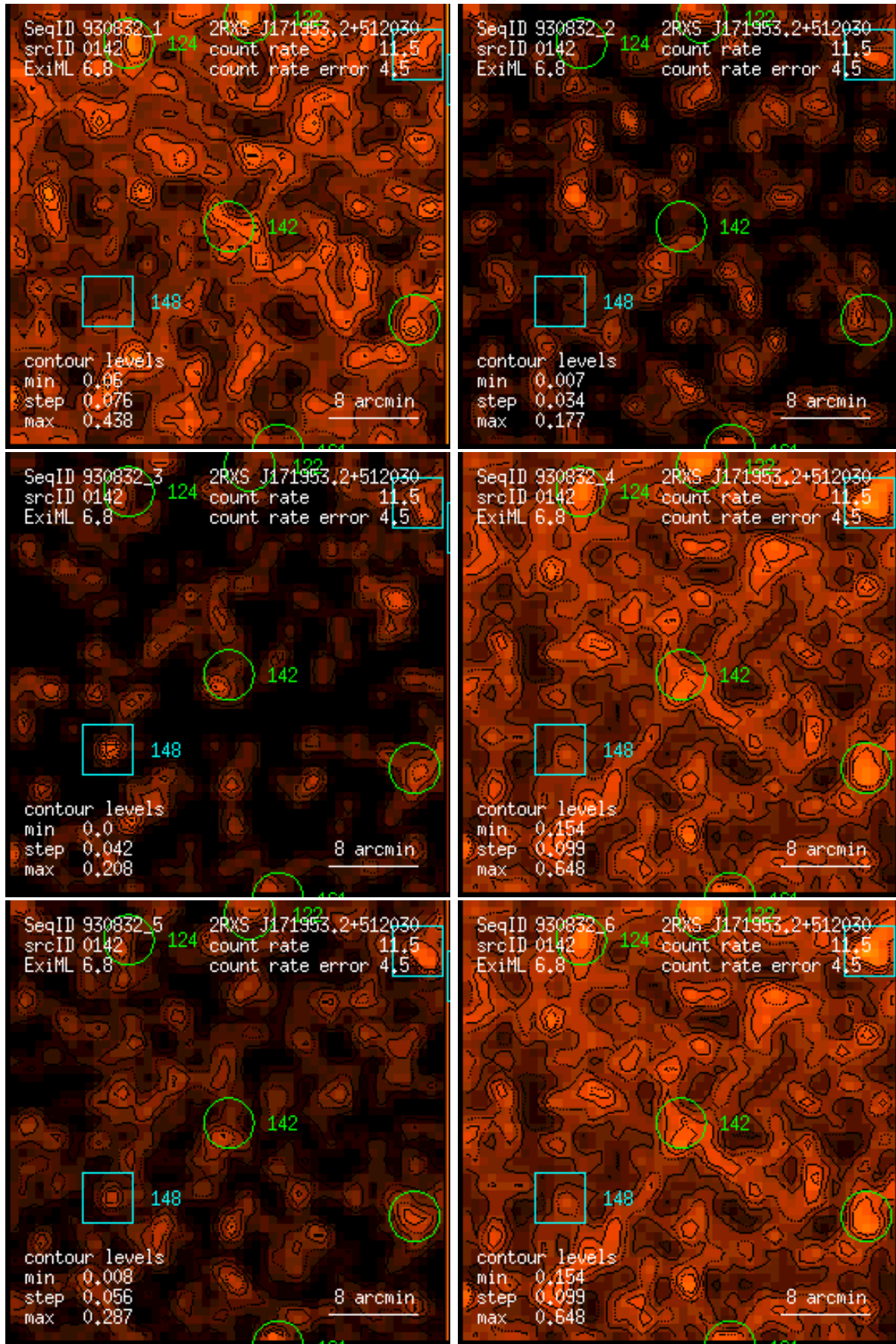
Figure 142: RASS 930832: detection 0142: band rate images, Gaussian filter: (1) PSPC channels 11 – 41, (2) 52 – 90, (3) 91 – 201, (4) 11 – 235, (5) 52 – 201, (6) 11 – 201. Broad band rates in counts/ks. Band rate contour levels in counts/ks/arcmin 2 .
