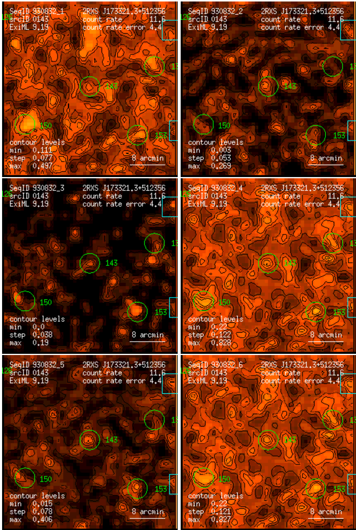
Figure 143: RASS 930832: detection 0143: band rate images, Gaussian filter: (1) PSPC channels 11 – 41, (2) 52 – 90, (3) 91 – 201, (4) 11 – 235, (5) 52 – 201, (6) 11 – 201. Broad band rates in counts/ks. Band rate contour levels in counts/ks/arcmin 2 .
