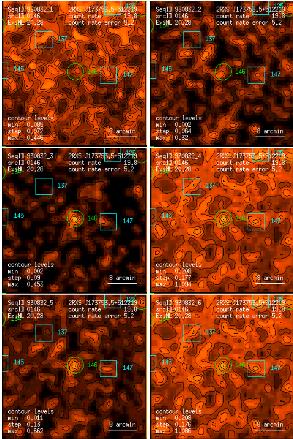
Figure 146: RASS 930832: detection 0146: band rate images, Gaussian filter: (1) PSPC channels 11 – 41, (2) 52 – 90, (3) 91 – 201, (4) 11 – 235, (5) 52 – 201, (6) 11 – 201. Broad band rates in counts/ks. Band rate contour levels in counts/ks/arcmin 2 .
