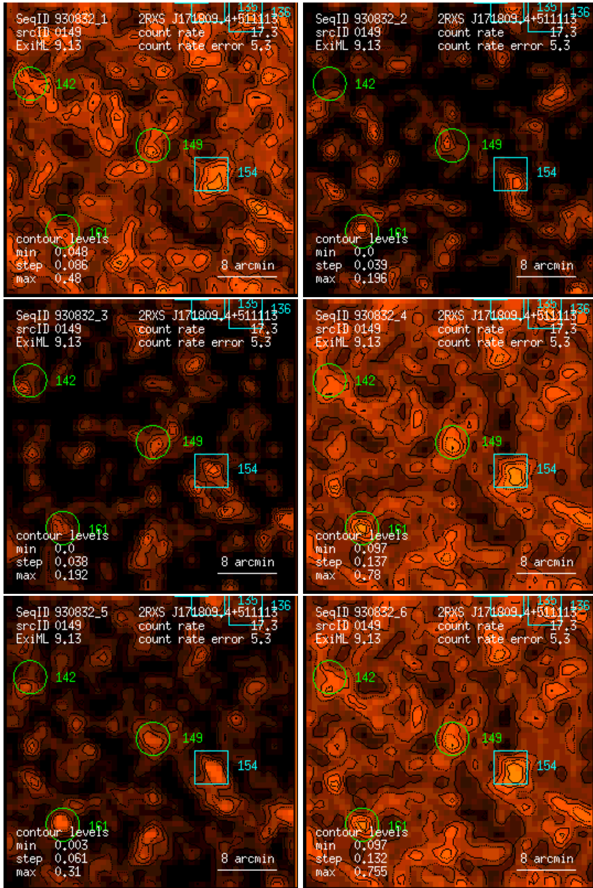
Figure 149: RASS 930832: detection 0149: band rate images, Gaussian filter: (1) PSPC channels 11 – 41, (2) 52 – 90, (3) 91 – 201, (4) 11 – 235, (5) 52 – 201, (6) 11 – 201. Broad band rates in counts/ks. Band rate contour levels in counts/ks/arcmin 2 .
