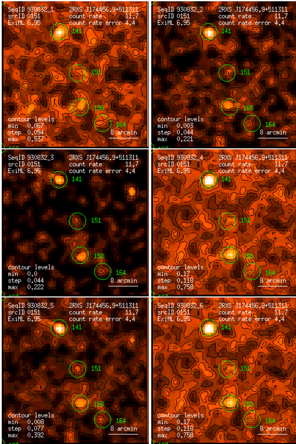
Figure 151: RASS 930832: detection 0151: band rate images, Gaussian filter: (1) PSPC channels 11 – 41, (2) 52 – 90, (3) 91 – 201, (4) 11 – 235, (5) 52 – 201, (6) 11 – 201. Broad band rates in counts/ks. Band rate contour levels in counts/ks/arcmin 2 .
