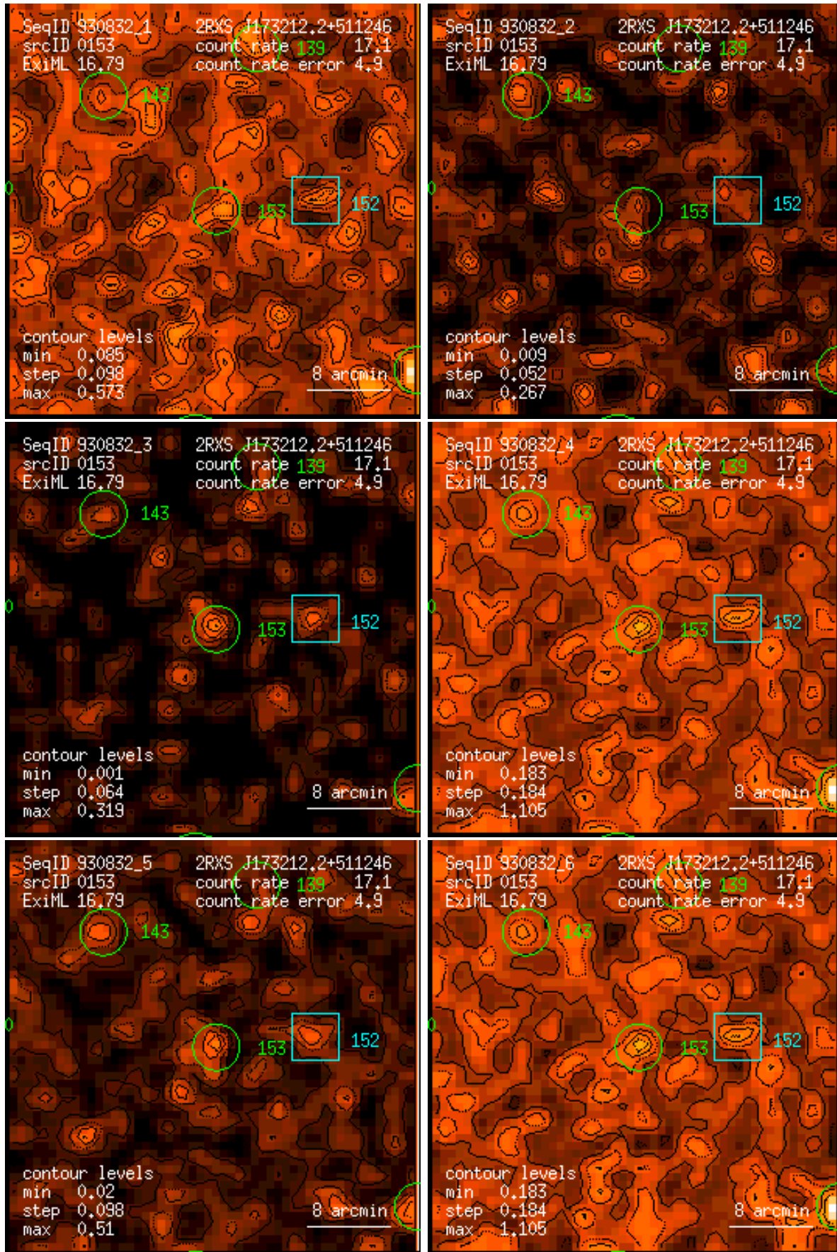
Figure 153: RASS 930832: detection 0153: band rate images, Gaussian filter: (1) PSPC channels 11 – 41, (2) 52 – 90, (3) 91 – 201, (4) 11 – 235, (5) 52 – 201, (6) 11 – 201. Broad band rates in counts/ks. Band rate contour levels in counts/ks/arcmin 2 .
