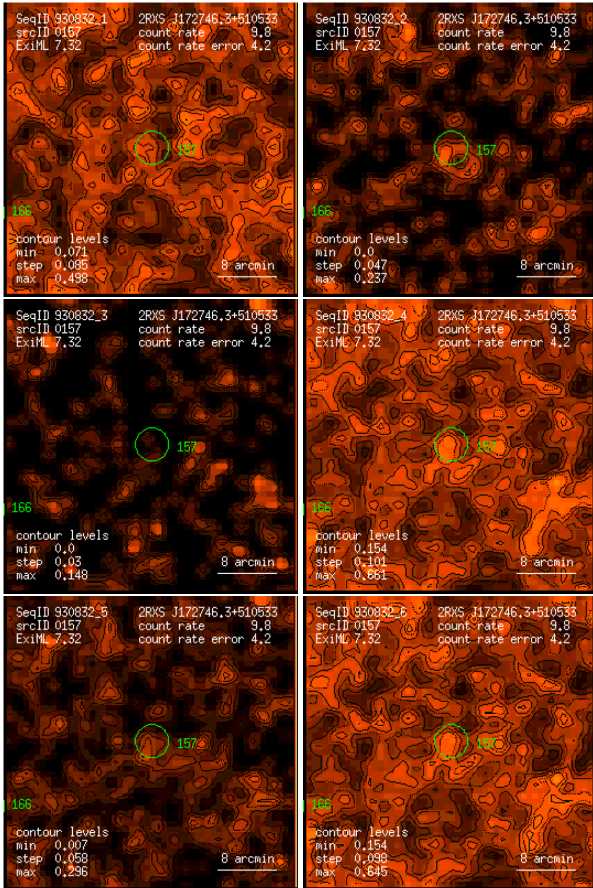
Figure 157: RASS 930832: detection 0157: band rate images, Gaussian filter: (1) PSPC channels 11 – 41, (2) 52 – 90, (3) 91 – 201, (4) 11 – 235, (5) 52 – 201, (6) 11 – 201. Broad band rates in counts/ks. Band rate contour levels in counts/ks/arcmin 2 .
