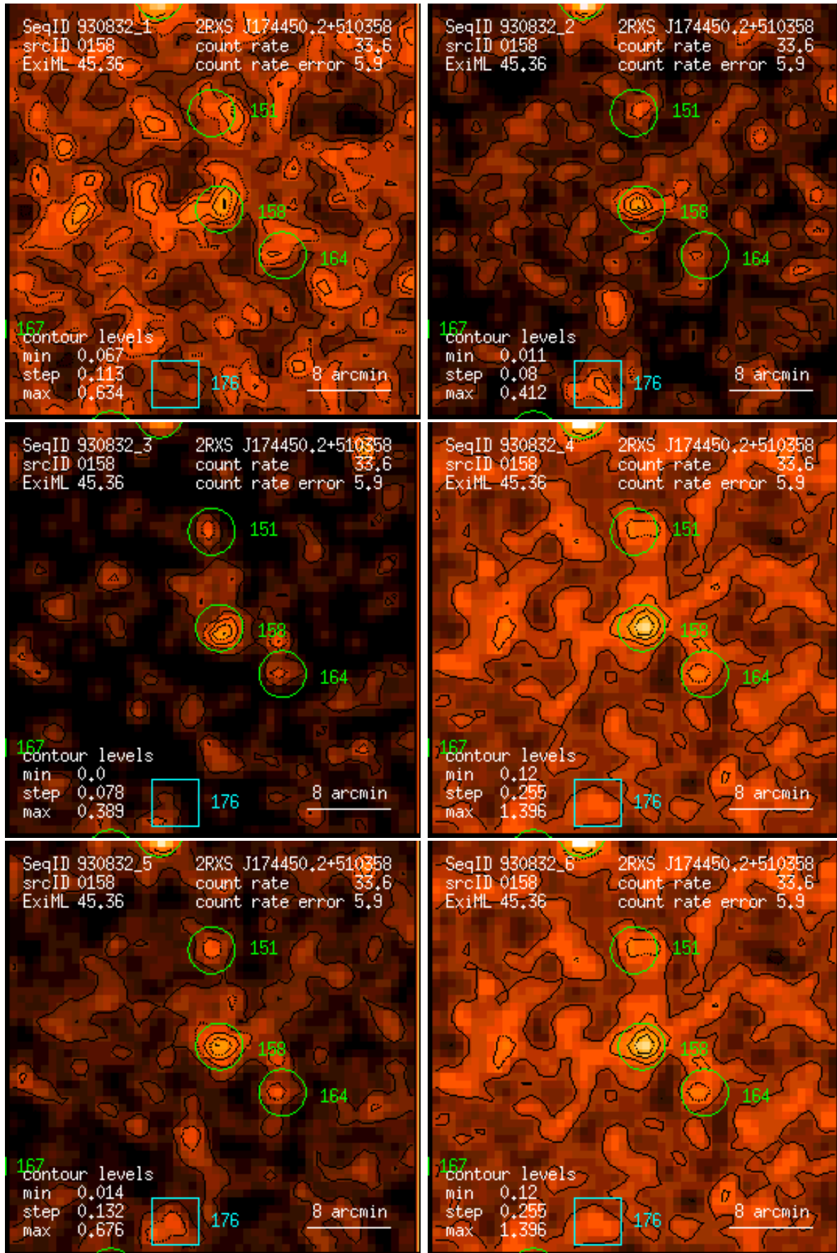
Figure 158: RASS 930832: detection 0158: band rate images, Gaussian filter: (1) PSPC channels 11 – 41, (2) 52 – 90, (3) 91 – 201, (4) 11 – 235, (5) 52 – 201, (6) 11 – 201. Broad band rates in counts/ks. Band rate contour levels in counts/ks/arcmin 2 .
