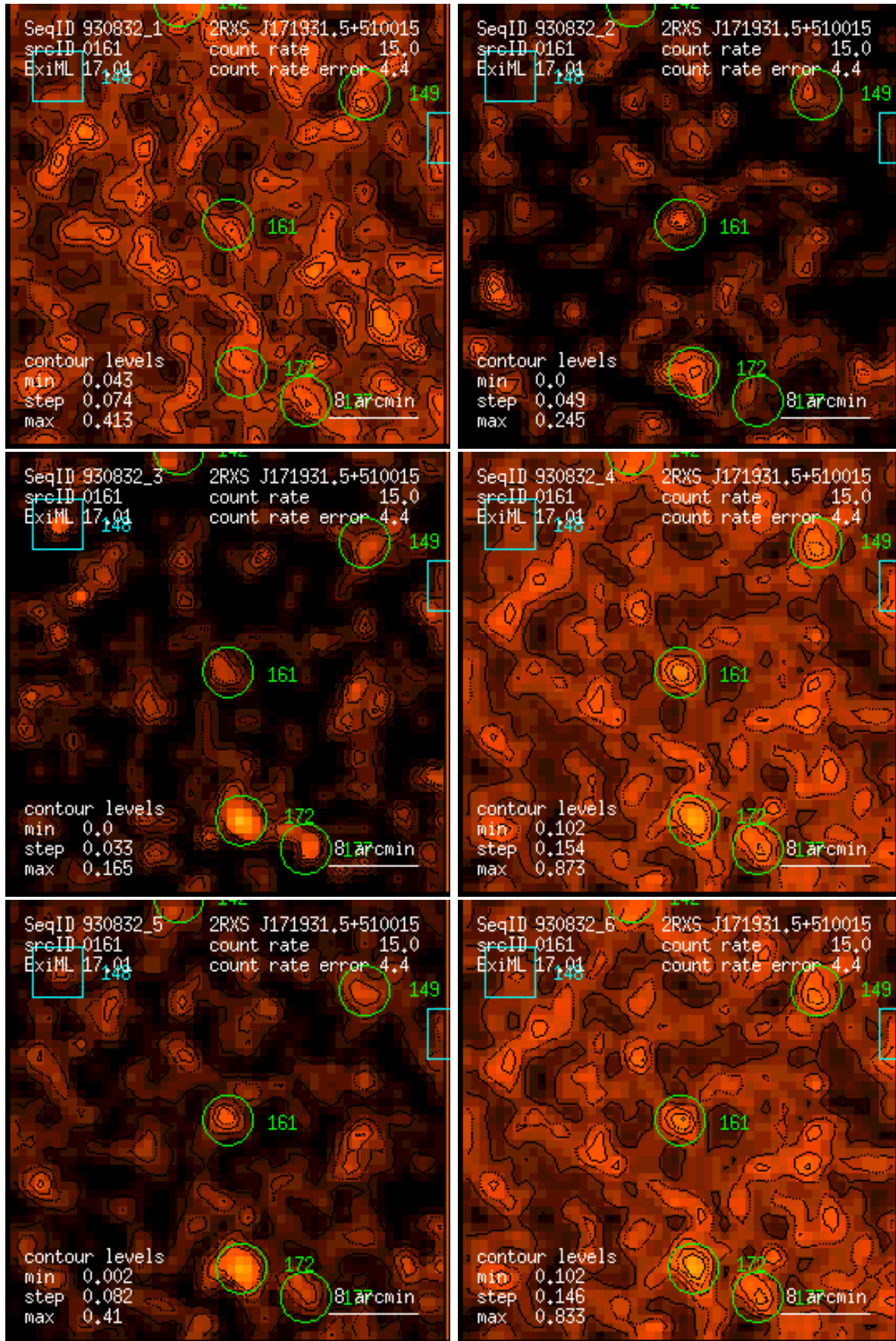
Figure 161: RASS 930832: detection 0161: band rate images, Gaussian filter: (1) PSPC channels 11 – 41, (2) 52 – 90, (3) 91 – 201, (4) 11 – 235, (5) 52 – 201, (6) 11 – 201. Broad band rates in counts/ks. Band rate contour levels in counts/ks/arcmin 2 .
