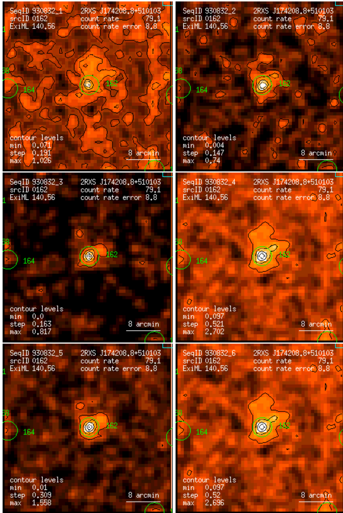
Figure 162: RASS 930832: detection 0162: band rate images, Gaussian filter: (1) PSPC channels 11 – 41, (2) 52 – 90, (3) 91 – 201, (4) 11 – 235, (5) 52 – 201, (6) 11 – 201. Broad band rates in counts/ks. Band rate contour levels in counts/ks/arcmin 2 .
