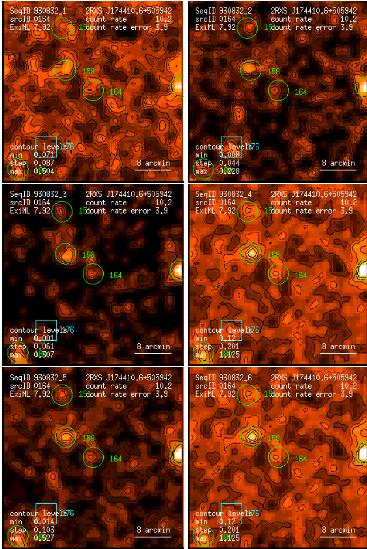
Figure 164: RASS 930832: detection 0164: band rate images, Gaussian filter: (1) PSPC channels 11 – 41, (2) 52 – 90, (3) 91 – 201, (4) 11 – 235, (5) 52 – 201, (6) 11 – 201. Broad band rates in counts/ks. Band rate contour levels in counts/ks/arcmin 2 .
