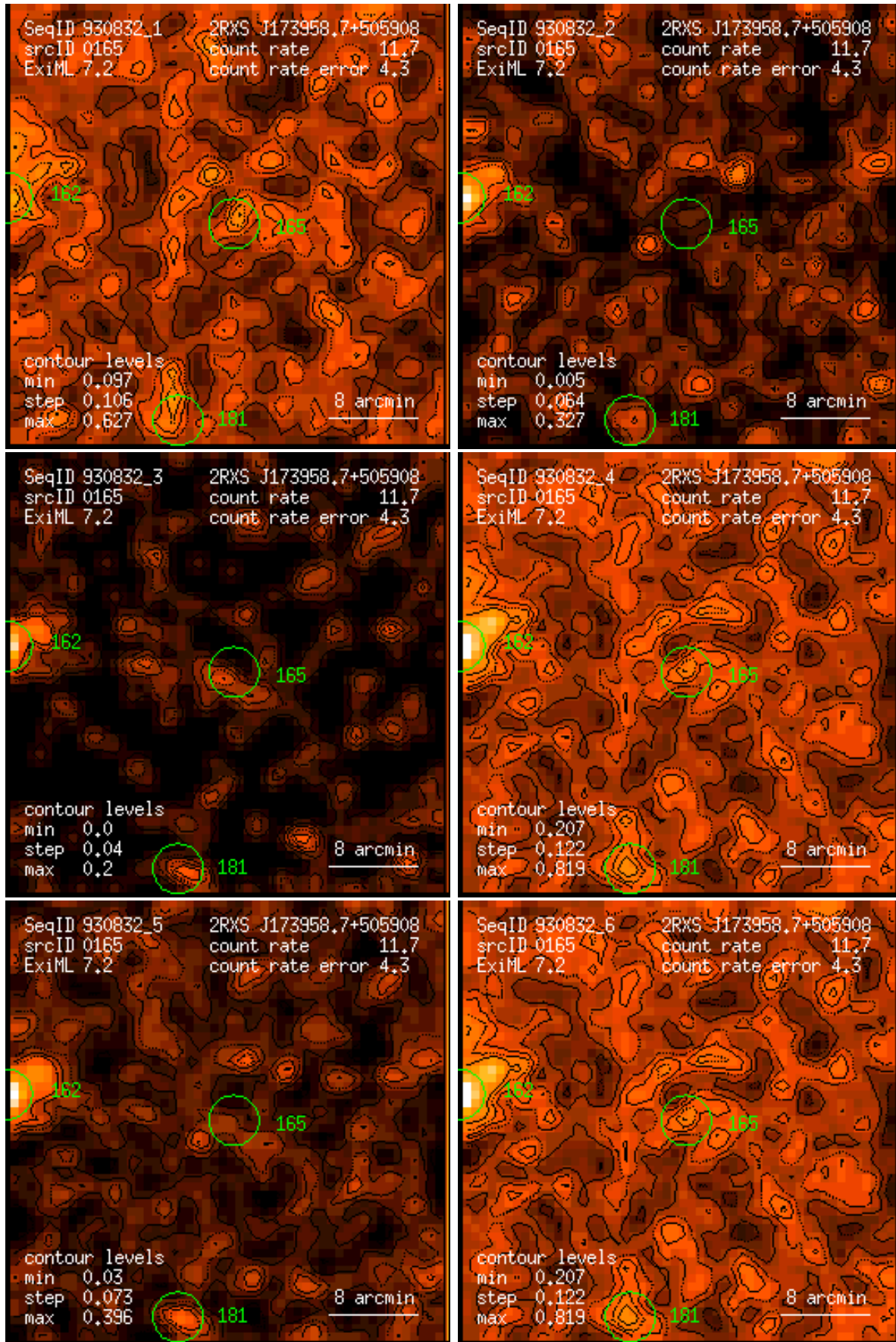
Figure 165: RASS 930832: detection 0165: band rate images, Gaussian filter: (1) PSPC channels 11 – 41, (2) 52 – 90, (3) 91 – 201, (4) 11 – 235, (5) 52 – 201, (6) 11 – 201. Broad band rates in counts/ks. Band rate contour levels in counts/ks/arcmin 2 .
