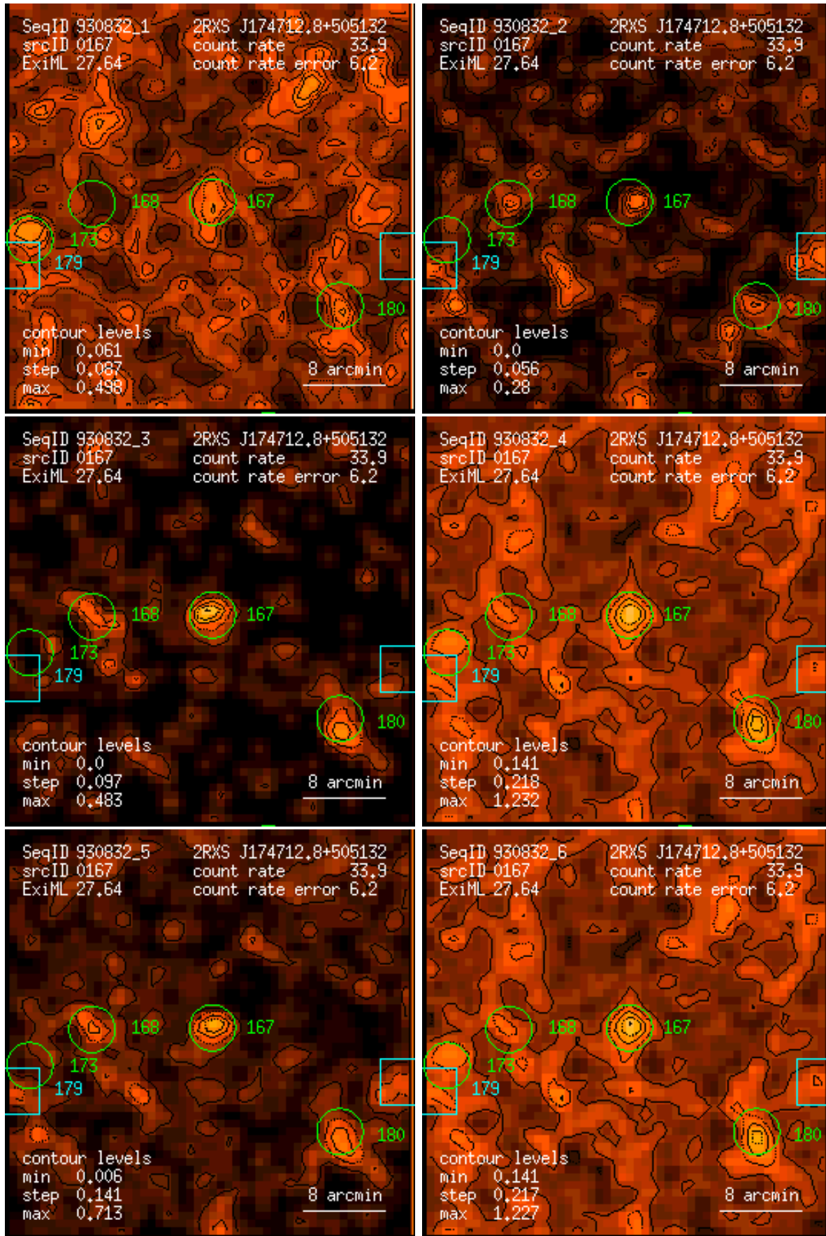
Figure 167: RASS 930832: detection 0167: band rate images, Gaussian filter: (1) PSPC channels 11 – 41, (2) 52 – 90, (3) 91 – 201, (4) 11 – 235, (5) 52 – 201, (6) 11 – 201. Broad band rates in counts/ks. Band rate contour levels in counts/ks/arcmin 2 .
