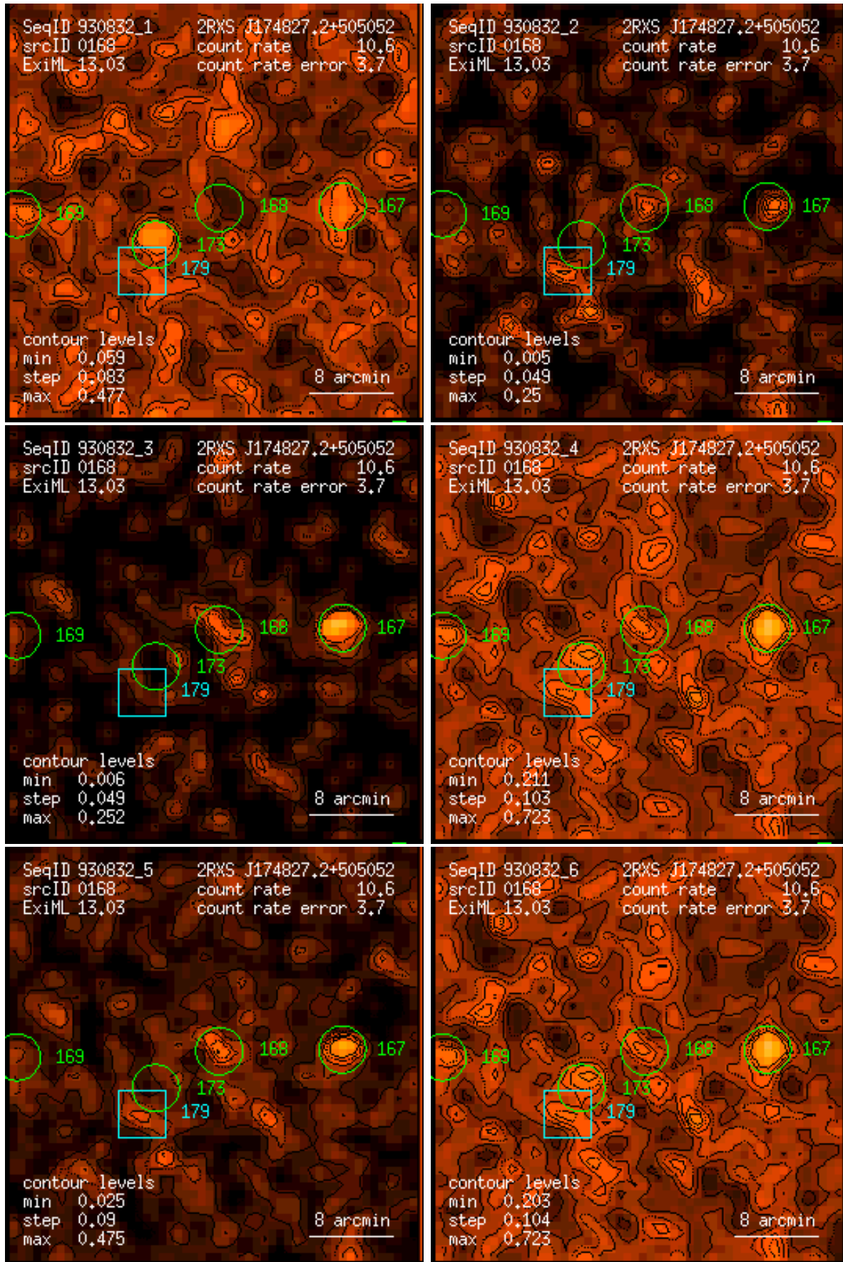
Figure 168: RASS 930832: detection 0168: band rate images, Gaussian filter: (1) PSPC channels 11 – 41, (2) 52 – 90, (3) 91 – 201, (4) 11 – 235, (5) 52 – 201, (6) 11 – 201. Broad band rates in counts/ks. Band rate contour levels in counts/ks/arcmin 2 .
