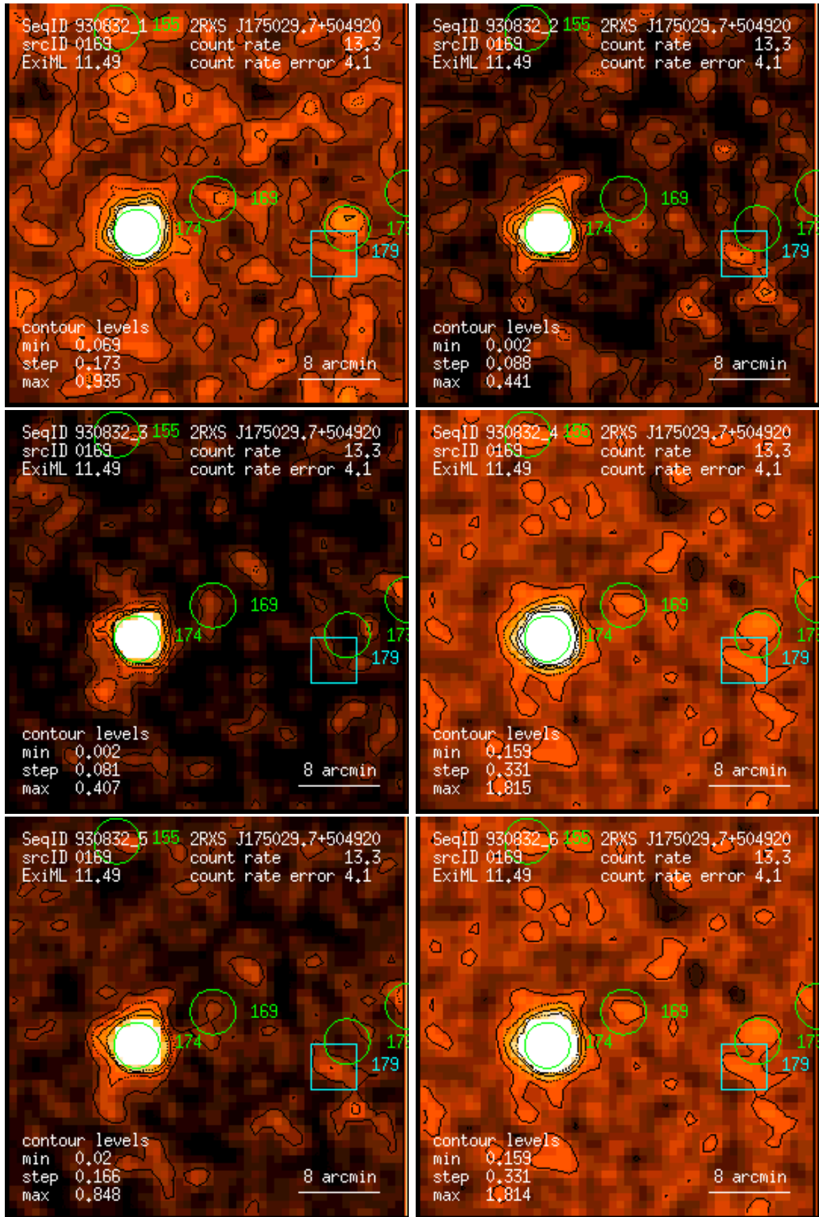
Figure 169: RASS 930832: detection 0169: band rate images, Gaussian filter: (1) PSPC channels 11 – 41, (2) 52 – 90, (3) 91 – 201, (4) 11 – 235, (5) 52 – 201, (6) 11 – 201. Broad band rates in counts/ks. Band rate contour levels in counts/ks/arcmin 2 .
