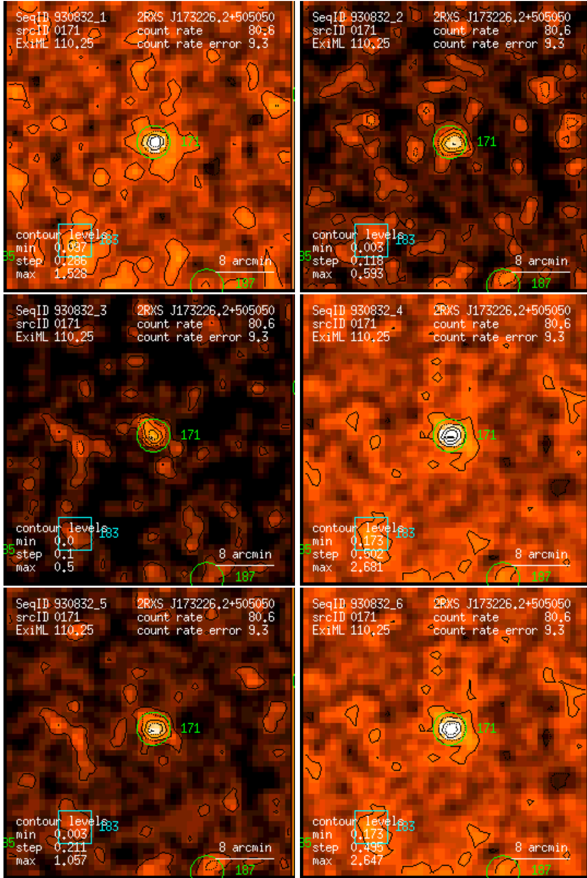
Figure 171: RASS 930832: detection 0171: band rate images, Gaussian filter: (1) PSPC channels 11 – 41, (2) 52 – 90, (3) 91 – 201, (4) 11 – 235, (5) 52 – 201, (6) 11 – 201. Broad band rates in counts/ks. Band rate contour levels in counts/ks/arcmin 2 .
