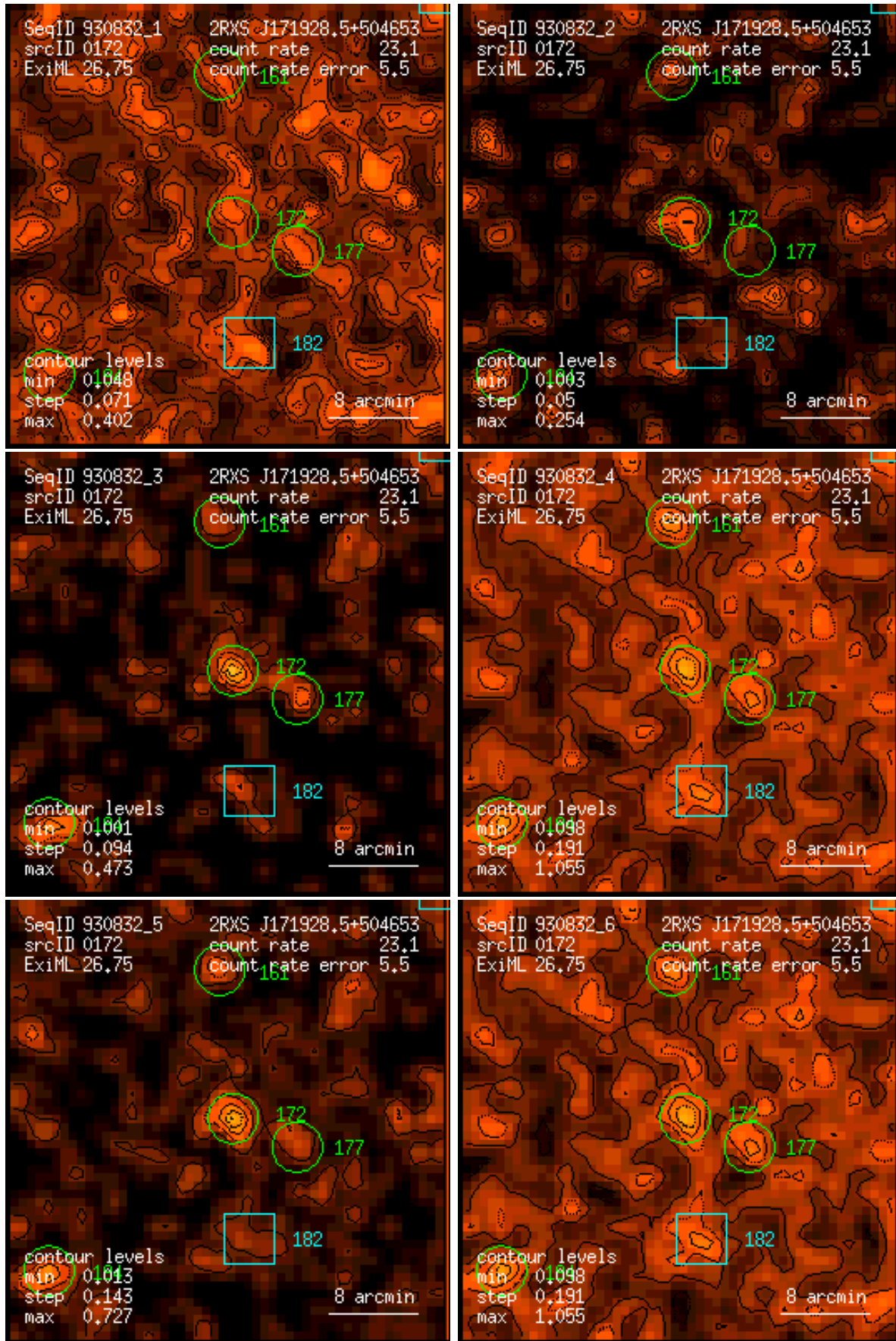
Figure 172: RASS 930832: detection 0172: band rate images, Gaussian filter: (1) PSPC channels 11 – 41, (2) 52 – 90, (3) 91 – 201, (4) 11 – 235, (5) 52 – 201, (6) 11 – 201. Broad band rates in counts/ks. Band rate contour levels in counts/ks/arcmin 2 .
