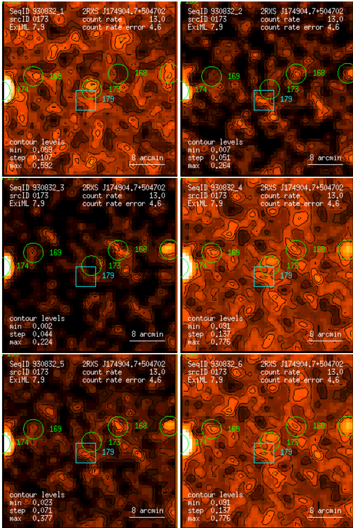
Figure 173: RASS 930832: detection 0173: band rate images, Gaussian filter: (1) PSPC channels 11 – 41, (2) 52 – 90, (3) 91 – 201, (4) 11 – 235, (5) 52 – 201, (6) 11 – 201. Broad band rates in counts/ks. Band rate contour levels in counts/ks/arcmin 2 .
