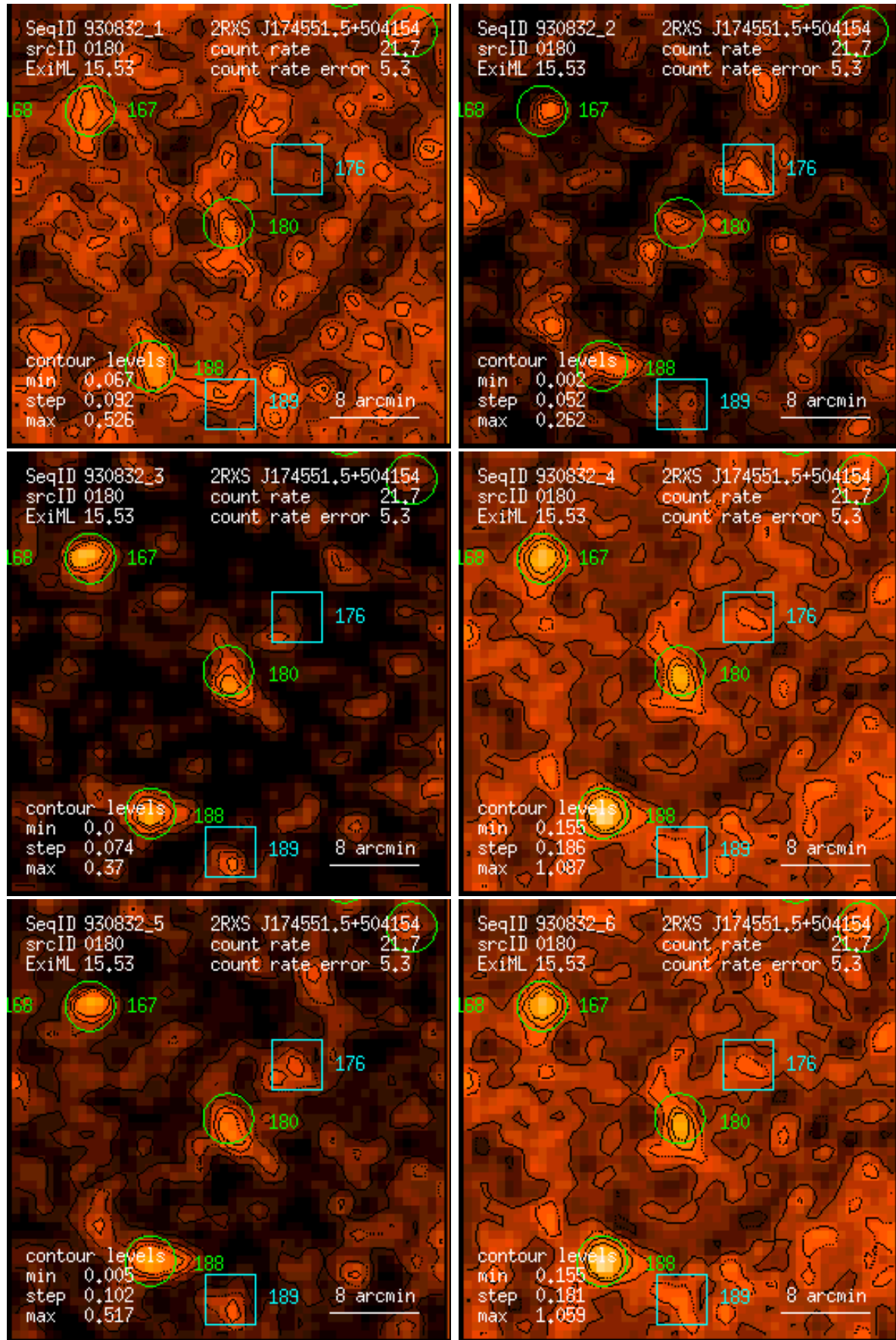
Figure 180: RASS 930832: detection 0180: band rate images, Gaussian filter: (1) PSPC channels 11 – 41, (2) 52 – 90, (3) 91 – 201, (4) 11 – 235, (5) 52 – 201, (6) 11 – 201. Broad band rates in counts/ks. Band rate contour levels in counts/ks/arcmin 2 .
