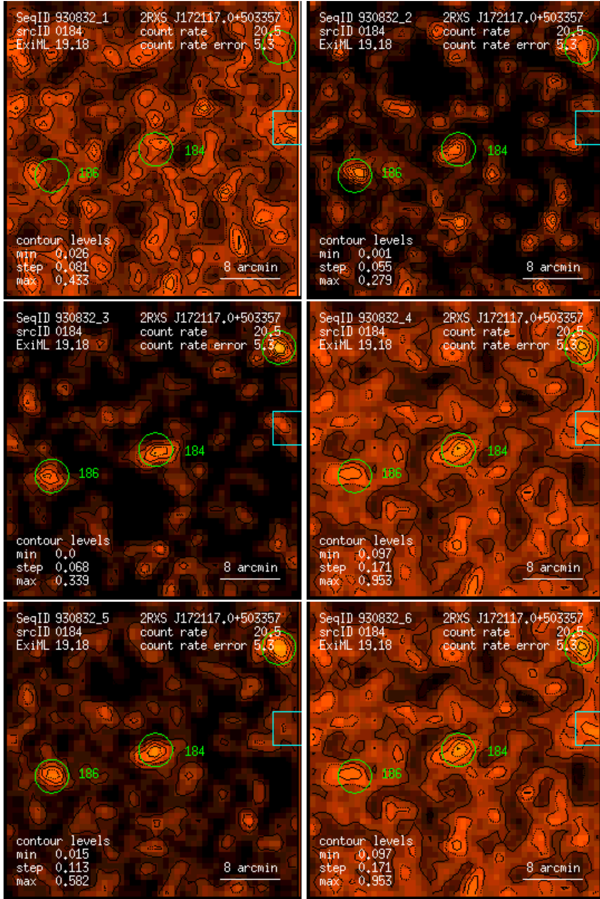
Figure 184: RASS 930832: detection 0184: band rate images, Gaussian filter: (1) PSPC channels 11 – 41, (2) 52 – 90, (3) 91 – 201, (4) 11 – 235, (5) 52 – 201, (6) 11 – 201. Broad band rates in counts/ks. Band rate contour levels in counts/ks/arcmin 2 .
