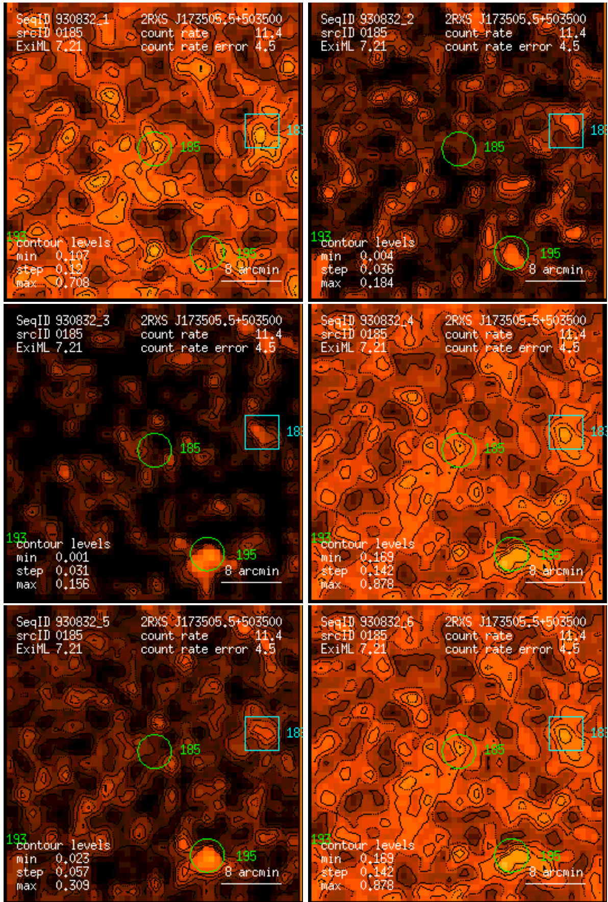
Figure 185: RASS 930832: detection 0185: band rate images, Gaussian filter: (1) PSPC channels 11 – 41, (2) 52 – 90, (3) 91 – 201, (4) 11 – 235, (5) 52 – 201, (6) 11 – 201. Broad band rates in counts/ks. Band rate contour levels in counts/ks/arcmin 2 .
