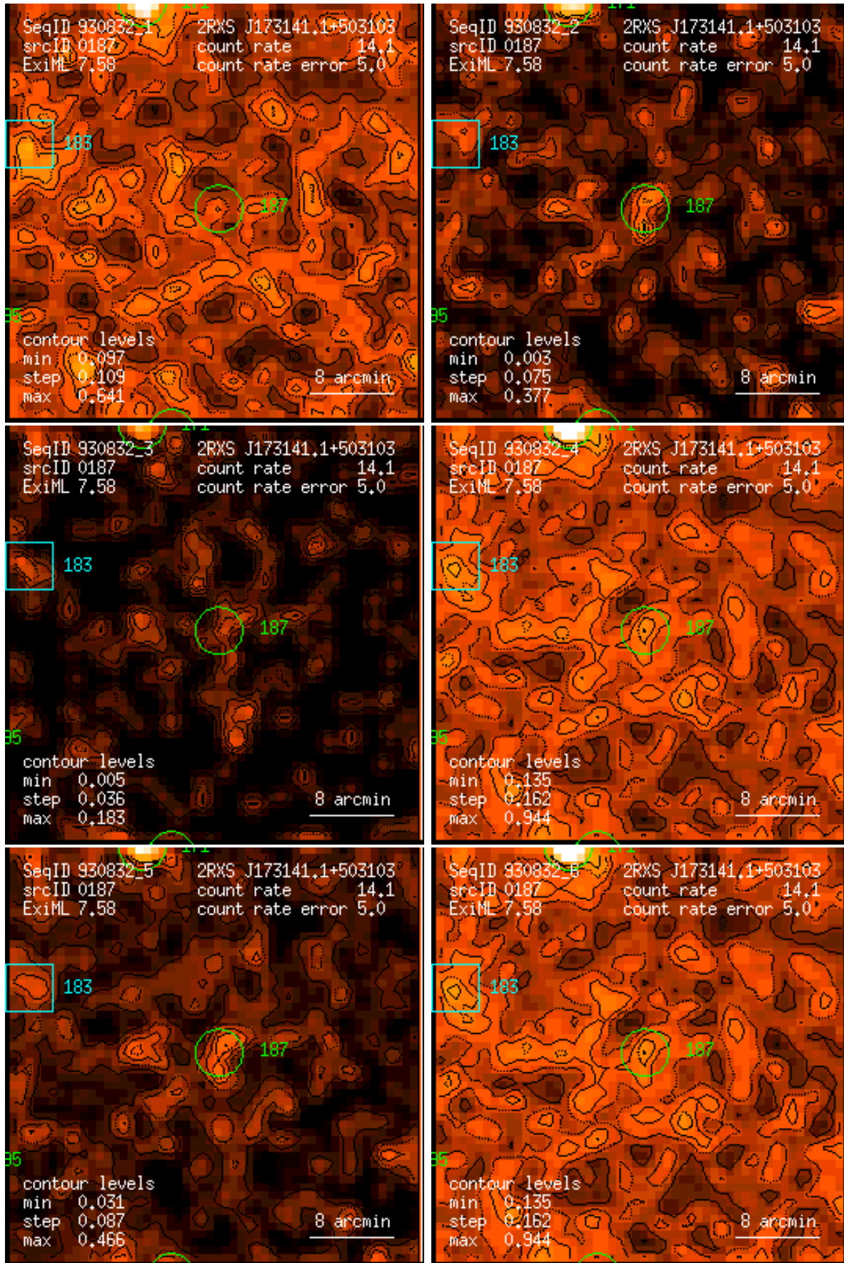
Figure 187: RASS 930832: detection 0187: band rate images, Gaussian filter: (1) PSPC channels 11 – 41, (2) 52 – 90, (3) 91 – 201, (4) 11 – 235, (5) 52 – 201, (6) 11 – 201. Broad band rates in counts/ks. Band rate contour levels in counts/ks/arcmin 2 .
