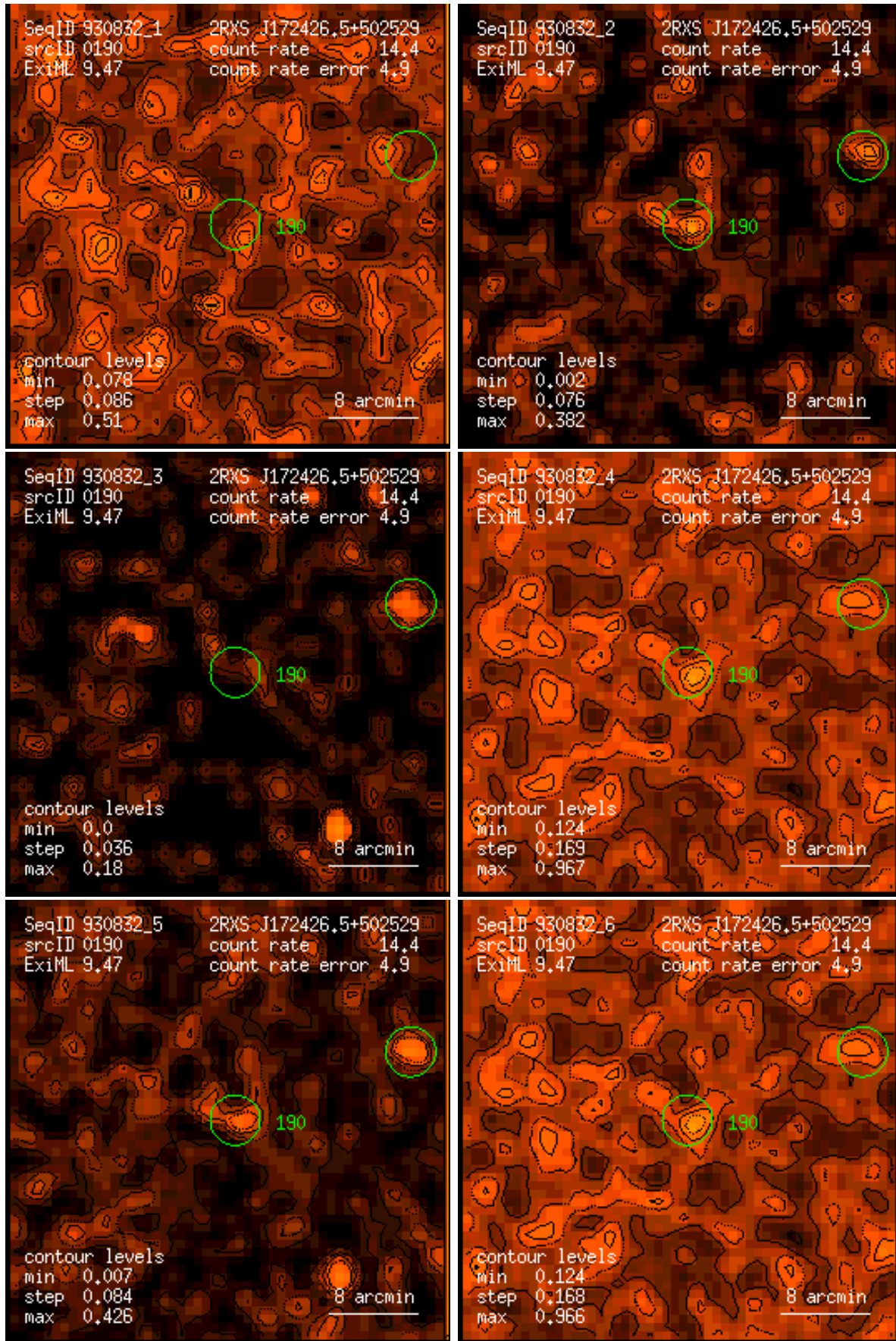
Figure 190: RASS 930832: detection 0190: band rate images, Gaussian filter: (1) PSPC channels 11 – 41, (2) 52 – 90, (3) 91 – 201, (4) 11 – 235, (5) 52 – 201, (6) 11 – 201. Broad band rates in counts/ks. Band rate contour levels in counts/ks/arcmin 2 .
