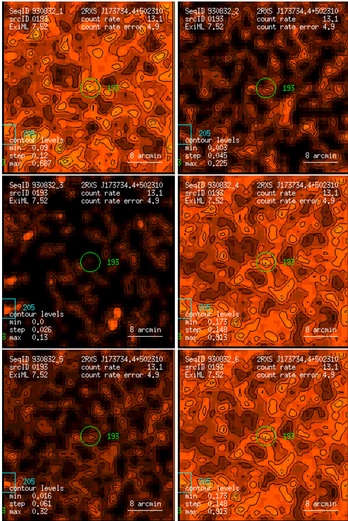
Figure 193: RASS 930832: detection 0193: band rate images, Gaussian filter: (1) PSPC channels 11 – 41, (2) 52 – 90, (3) 91 – 201, (4) 11 – 235, (5) 52 – 201, (6) 11 – 201. Broad band rates in counts/ks. Band rate contour levels in counts/ks/arcmin 2 .
