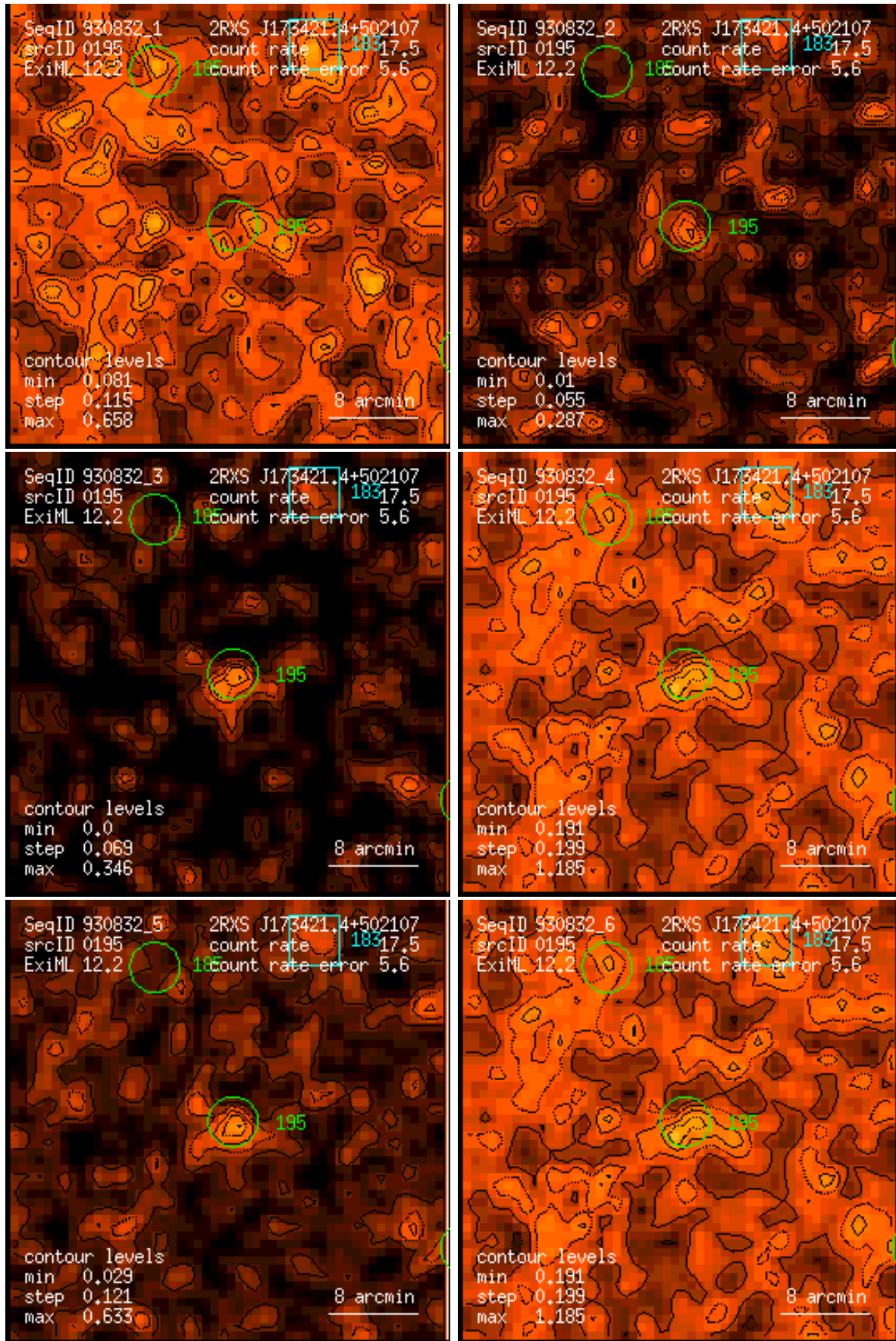
Figure 195: RASS 930832: detection 0195: band rate images, Gaussian filter: (1) PSPC channels 11 – 41, (2) 52 – 90, (3) 91 – 201, (4) 11 – 235, (5) 52 – 201, (6) 11 – 201. Broad band rates in counts/ks. Band rate contour levels in counts/ks/arcmin 2 .
