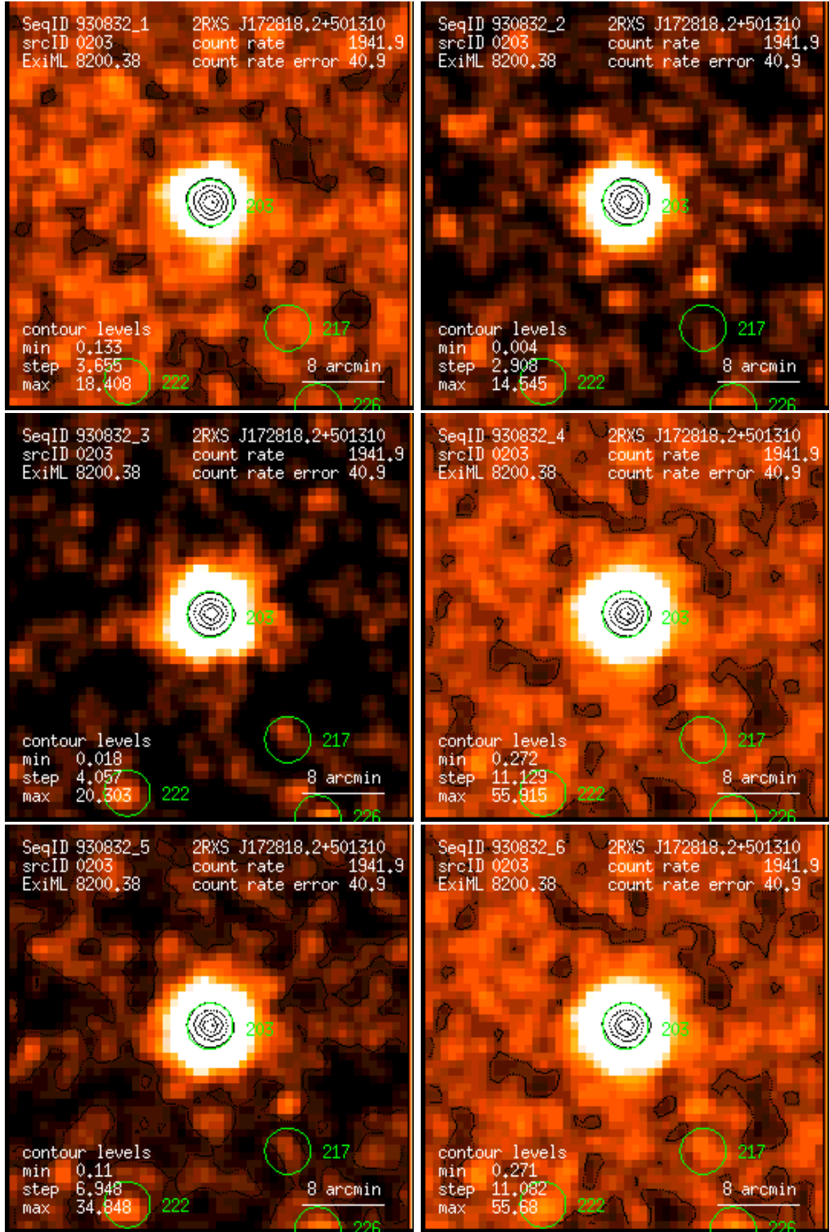
Figure 203: RASS 930832: detection 0203: band rate images, Gaussian filter: (1) PSPC channels 11 – 41, (2) 52 – 90, (3) 91 – 201, (4) 11 – 235, (5) 52 – 201, (6) 11 – 201. Broad band rates in counts/ks. Band rate contour levels in counts/ks/arcmin 2 .
