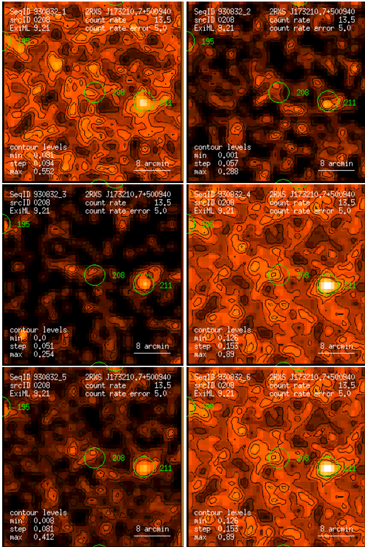
Figure 208: RASS 930832: detection 0208: band rate images, Gaussian filter: (1) PSPC channels 11 – 41, (2) 52 – 90, (3) 91 – 201, (4) 11 – 235, (5) 52 – 201, (6) 11 – 201. Broad band rates in counts/ks. Band rate contour levels in counts/ks/arcmin 2 .
