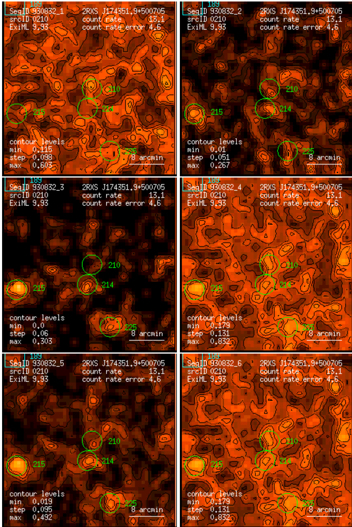
Figure 210: RASS 930832: detection 0210: band rate images, Gaussian filter: (1) PSPC channels 11 – 41, (2) 52 – 90, (3) 91 – 201, (4) 11 – 235, (5) 52 – 201, (6) 11 – 201. Broad band rates in counts/ks. Band rate contour levels in counts/ks/arcmin 2 .
