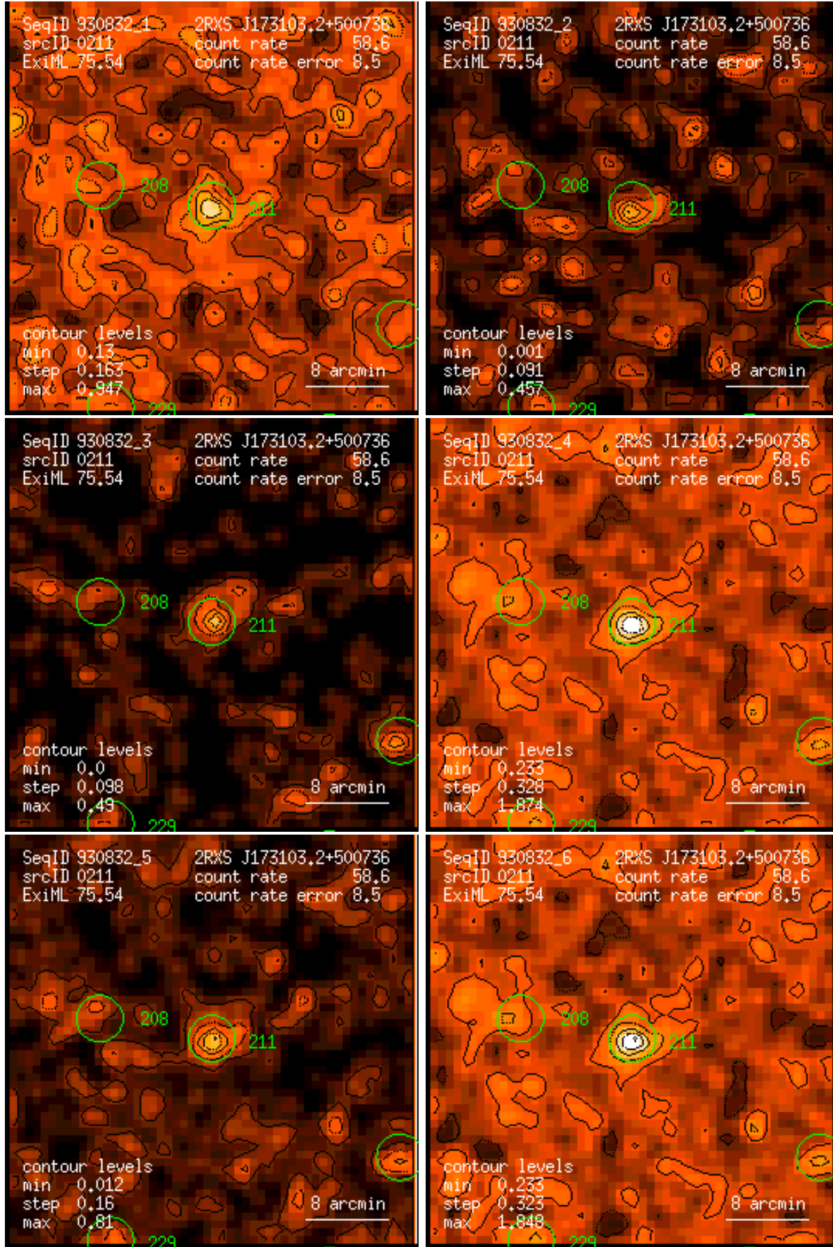
Figure 211: RASS 930832: detection 0211: band rate images, Gaussian filter: (1) PSPC channels 11 – 41, (2) 52 – 90, (3) 91 – 201, (4) 11 – 235, (5) 52 – 201, (6) 11 – 201. Broad band rates in counts/ks. Band rate contour levels in counts/ks/arcmin 2 .
