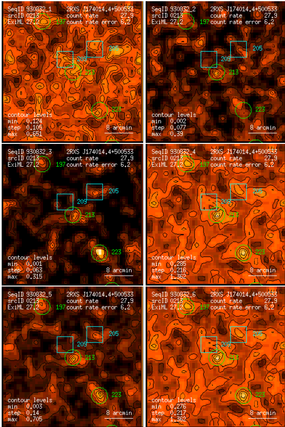
Figure 213: RASS 930832: detection 0213: band rate images, Gaussian filter: (1) PSPC channels 11 – 41, (2) 52 – 90, (3) 91 – 201, (4) 11 – 235, (5) 52 – 201, (6) 11 – 201. Broad band rates in counts/ks. Band rate contour levels in counts/ks/arcmin 2 .
