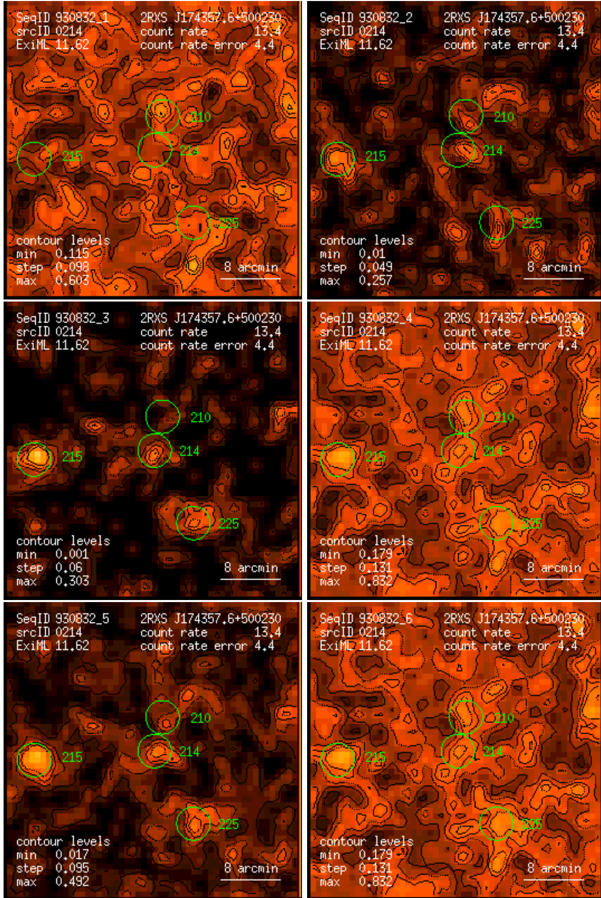
Figure 214: RASS 930832: detection 0214: band rate images, Gaussian filter: (1) PSPC channels 11 – 41, (2) 52 – 90, (3) 91 – 201, (4) 11 – 235, (5) 52 – 201, (6) 11 – 201. Broad band rates in counts/ks. Band rate contour levels in counts/ks/arcmin 2 .
