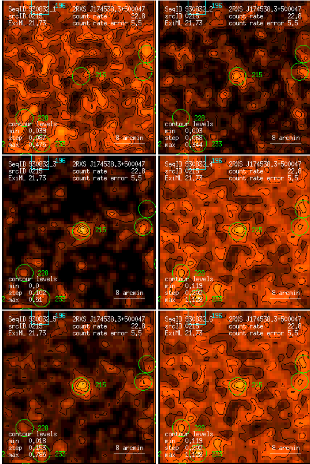
Figure 215: RASS 930832: detection 0215: band rate images, Gaussian filter: (1) PSPC channels 11 – 41, (2) 52 – 90, (3) 91 – 201, (4) 11 – 235, (5) 52 – 201, (6) 11 – 201. Broad band rates in counts/ks. Band rate contour levels in counts/ks/arcmin 2 .
