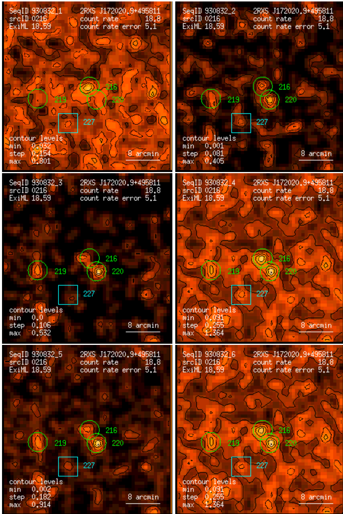
Figure 216: RASS 930832: detection 0216: band rate images, Gaussian filter: (1) PSPC channels 11 – 41, (2) 52 – 90, (3) 91 – 201, (4) 11 – 235, (5) 52 – 201, (6) 11 – 201. Broad band rates in counts/ks. Band rate contour levels in counts/ks/arcmin 2 .
