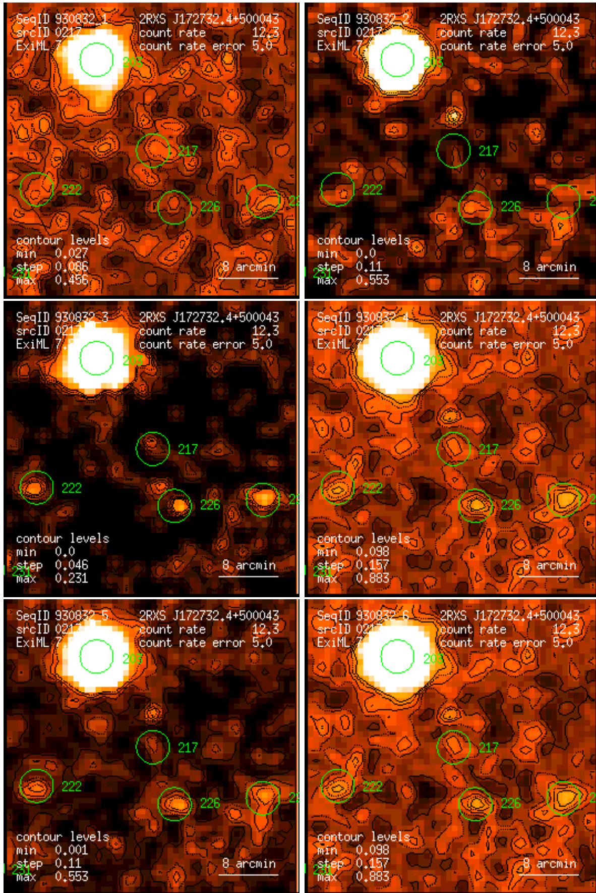
Figure 217: RASS 930832: detection 0217: band rate images, Gaussian filter: (1) PSPC channels 11 – 41, (2) 52 – 90, (3) 91 – 201, (4) 11 – 235, (5) 52 – 201, (6) 11 – 201. Broad band rates in counts/ks. Band rate contour levels in counts/ks/arcmin 2 .
