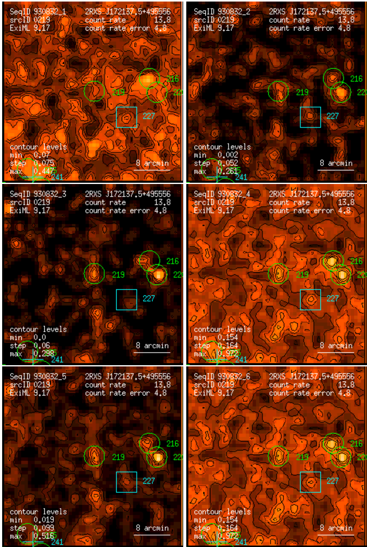
Figure 219: RASS 930832: detection 0219: band rate images, Gaussian filter: (1) PSPC channels 11 – 41, (2) 52 – 90, (3) 91 – 201, (4) 11 – 235, (5) 52 – 201, (6) 11 – 201. Broad band rates in counts/ks. Band rate contour levels in counts/ks/arcmin 2 .
