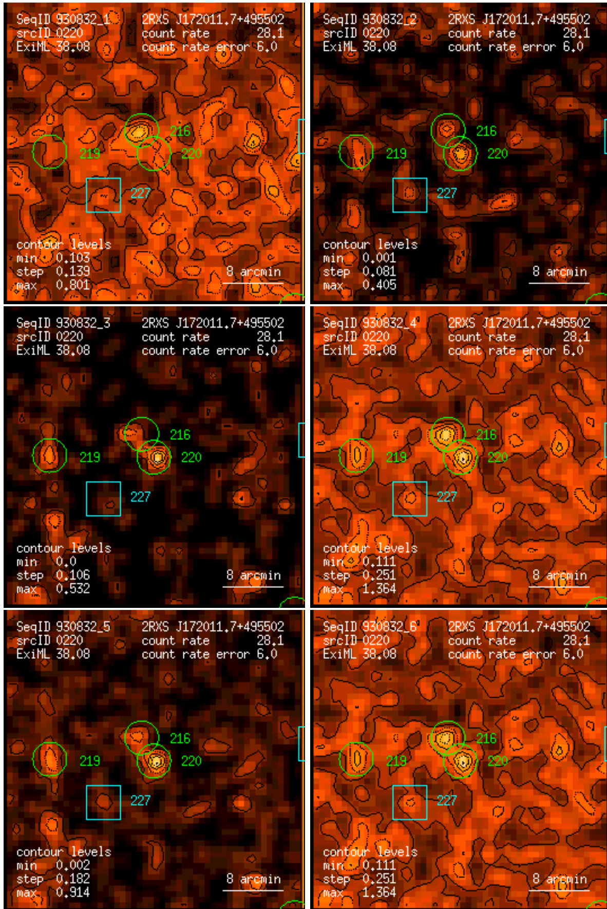
Figure 220: RASS 930832: detection 0220: band rate images, Gaussian filter: (1) PSPC channels 11 – 41, (2) 52 – 90, (3) 91 – 201, (4) 11 – 235, (5) 52 – 201, (6) 11 – 201. Broad band rates in counts/ks. Band rate contour levels in counts/ks/arcmin 2 .
