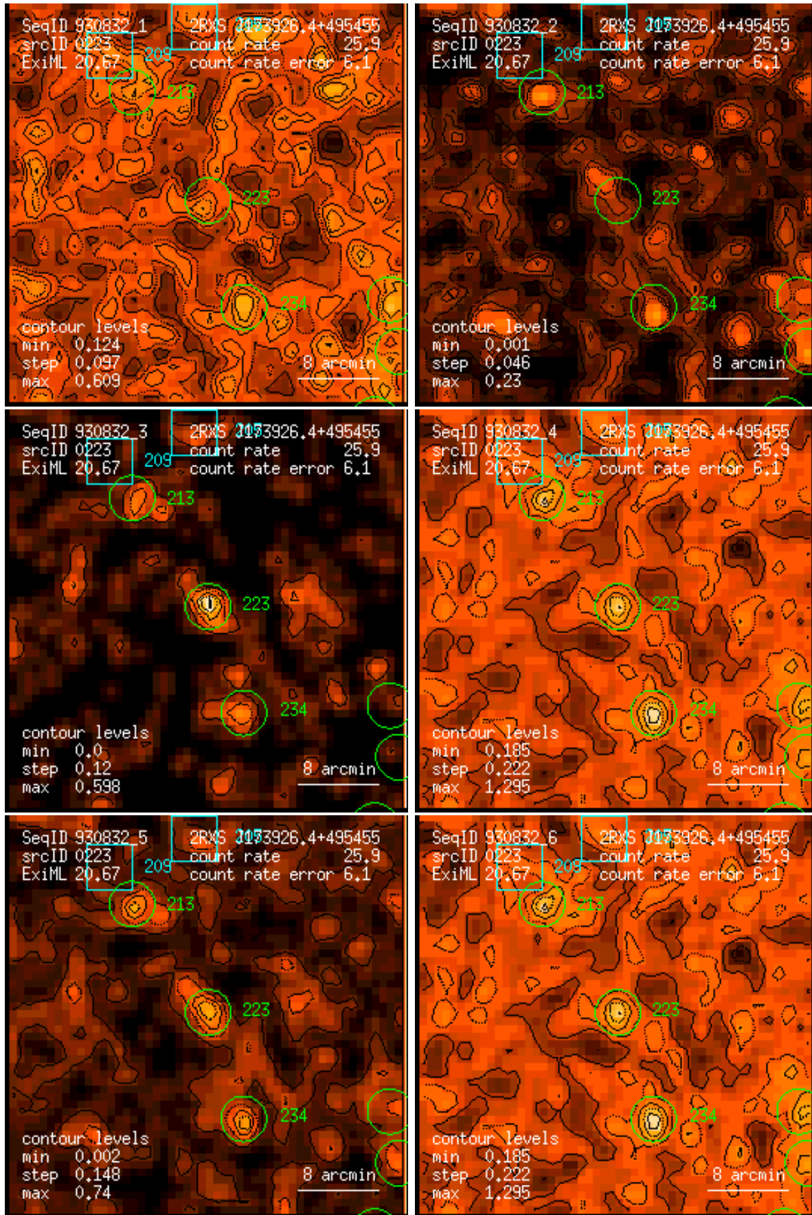
Figure 223: RASS 930832: detection 0223: band rate images, Gaussian filter: (1) PSPC channels 11 – 41, (2) 52 – 90, (3) 91 – 201, (4) 11 – 235, (5) 52 – 201, (6) 11 – 201. Broad band rates in counts/ks. Band rate contour levels in counts/ks/arcmin 2 .
