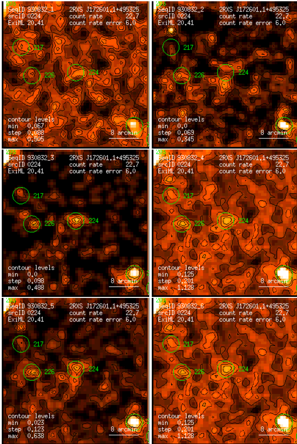
Figure 224: RASS 930832: detection 0224: band rate images, Gaussian filter: (1) PSPC channels 11 – 41, (2) 52 – 90, (3) 91 – 201, (4) 11 – 235, (5) 52 – 201, (6) 11 – 201. Broad band rates in counts/ks. Band rate contour levels in counts/ks/arcmin 2 .
