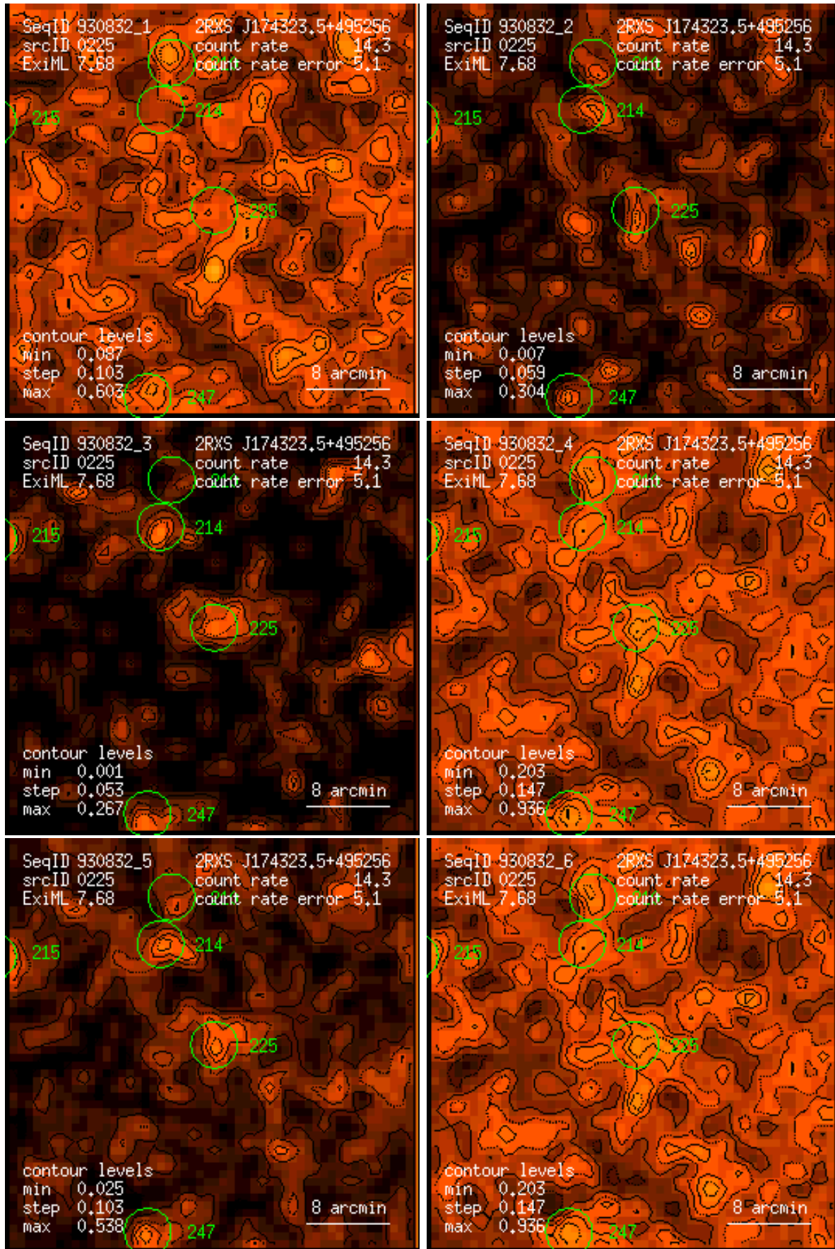
Figure 225: RASS 930832: detection 0225: band rate images, Gaussian filter: (1) PSPC channels 11 – 41, (2) 52 – 90, (3) 91 – 201, (4) 11 – 235, (5) 52 – 201, (6) 11 – 201. Broad band rates in counts/ks. Band rate contour levels in counts/ks/arcmin 2 .
