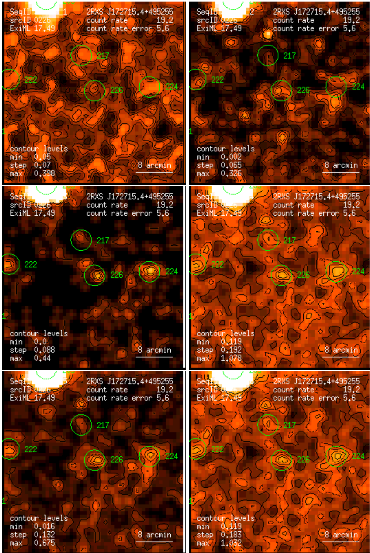
Figure 226: RASS 930832: detection 0226: band rate images, Gaussian filter: (1) PSPC channels 11 – 41, (2) 52 – 90, (3) 91 – 201, (4) 11 – 235, (5) 52 – 201, (6) 11 – 201. Broad band rates in counts/ks. Band rate contour levels in counts/ks/arcmin 2 .
