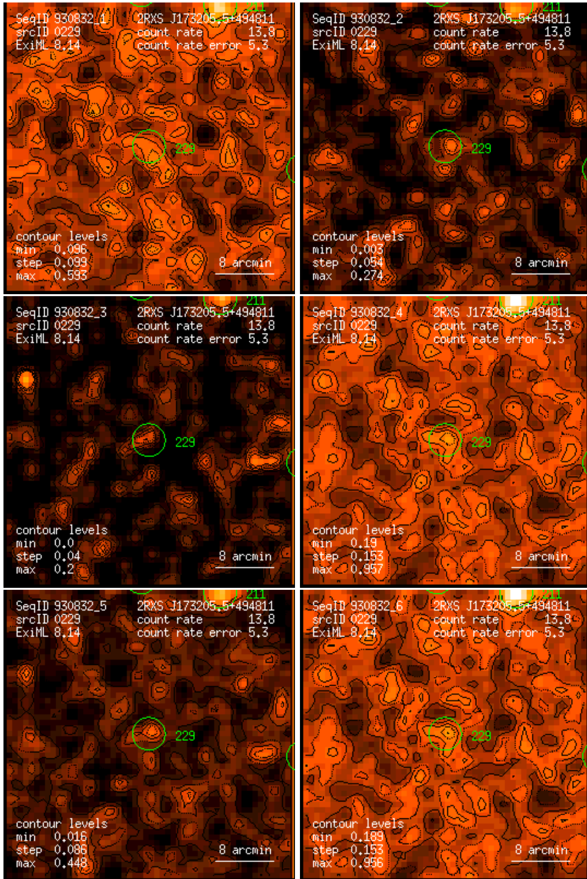
Figure 229: RASS 930832: detection 0229: band rate images, Gaussian filter: (1) PSPC channels 11 – 41, (2) 52 – 90, (3) 91 – 201, (4) 11 – 235, (5) 52 – 201, (6) 11 – 201. Broad band rates in counts/ks. Band rate contour levels in counts/ks/arcmin 2 .
