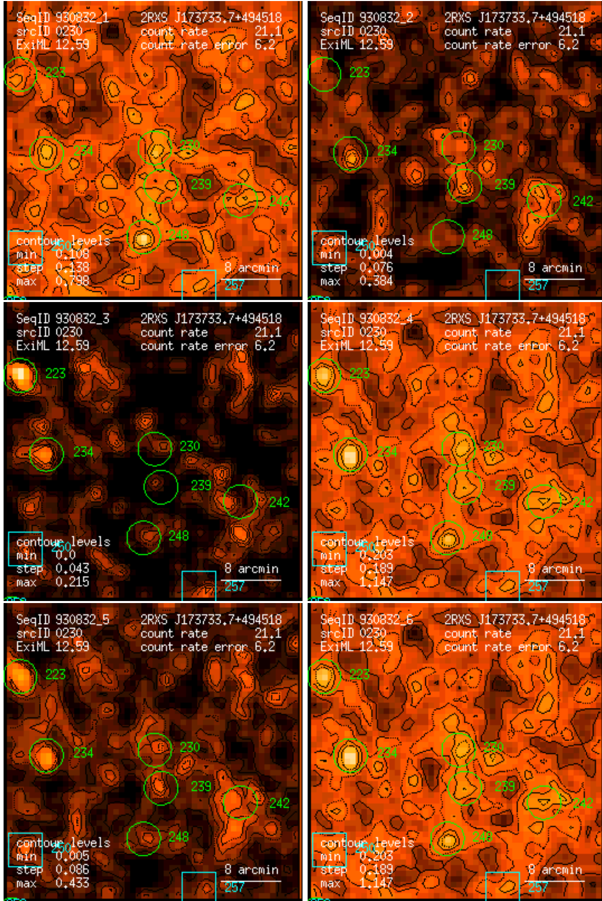
Figure 230: RASS 930832: detection 0230: band rate images, Gaussian filter: (1) PSPC channels 11 – 41, (2) 52 – 90, (3) 91 – 201, (4) 11 – 235, (5) 52 – 201, (6) 11 – 201. Broad band rates in counts/ks. Band rate contour levels in counts/ks/arcmin 2 .
