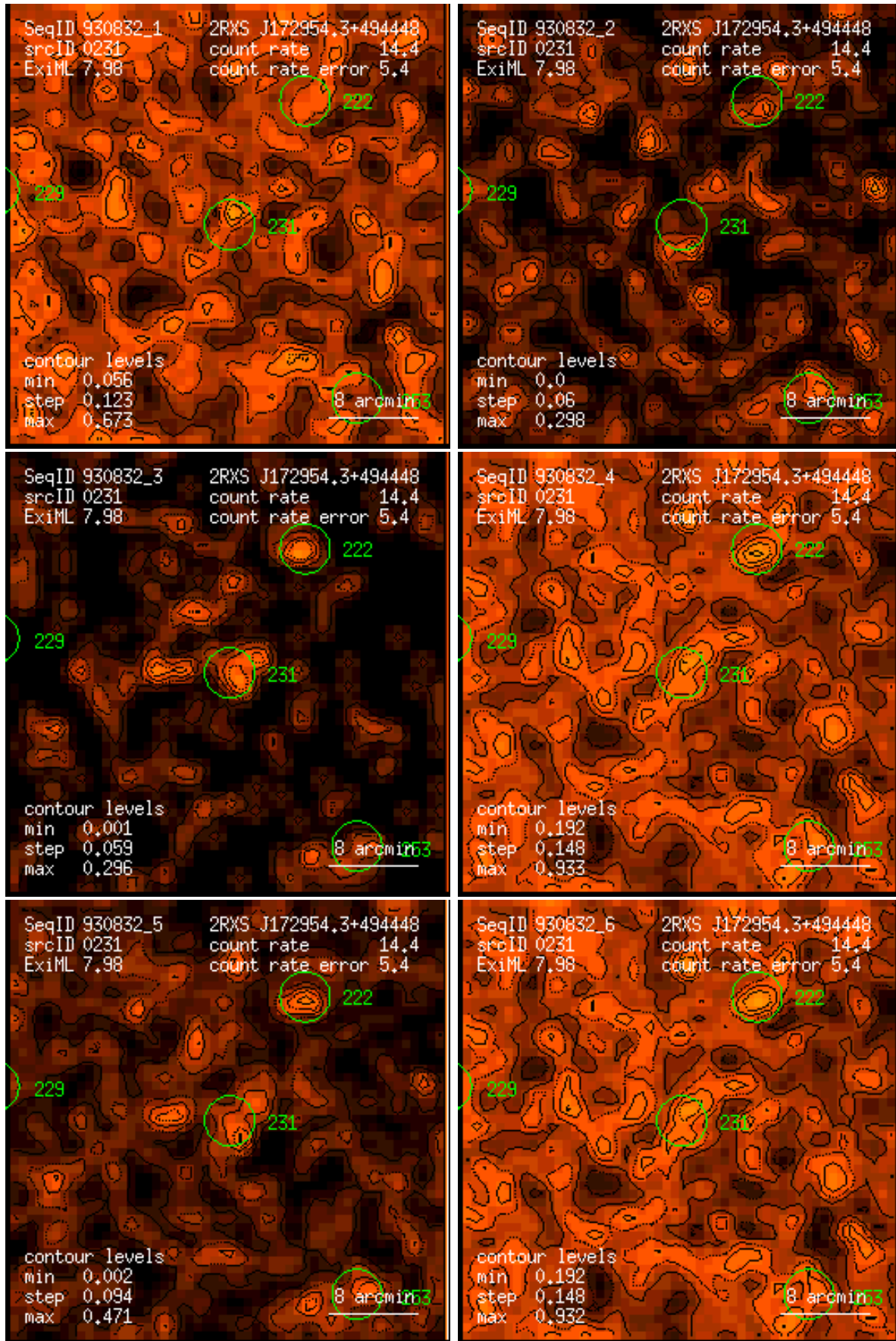
Figure 231: RASS 930832: detection 0231: band rate images, Gaussian filter: (1) PSPC channels 11 – 41, (2) 52 – 90, (3) 91 – 201, (4) 11 – 235, (5) 52 – 201, (6) 11 – 201. Broad band rates in counts/ks. Band rate contour levels in counts/ks/arcmin 2 .
