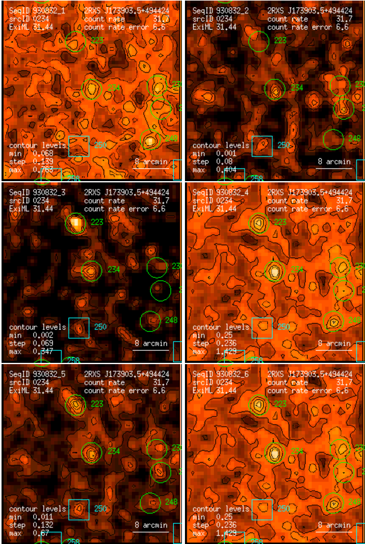
Figure 234: RASS 930832: detection 0234: band rate images, Gaussian filter: (1) PSPC channels 11 – 41, (2) 52 – 90, (3) 91 – 201, (4) 11 – 235, (5) 52 – 201, (6) 11 – 201. Broad band rates in counts/ks. Band rate contour levels in counts/ks/arcmin 2 .
