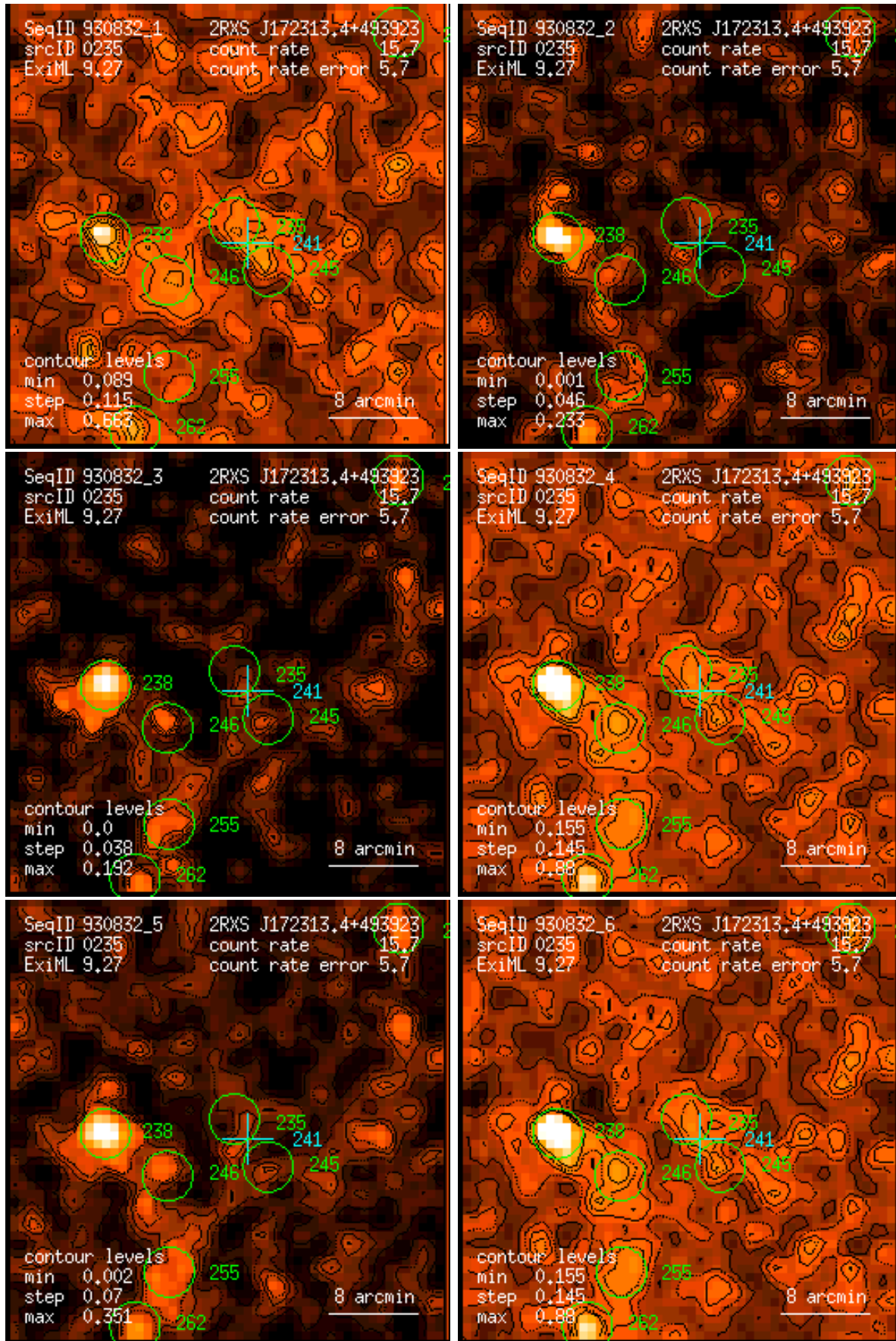
Figure 235: RASS 930832: detection 0235: band rate images, Gaussian filter: (1) PSPC channels 11 – 41, (2) 52 – 90, (3) 91 – 201, (4) 11 – 235, (5) 52 – 201, (6) 11 – 201. Broad band rates in counts/ks. Band rate contour levels in counts/ks/arcmin 2 .
