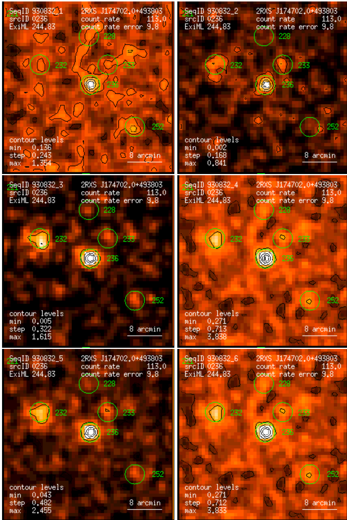
Figure 236: RASS 930832: detection 0236: band rate images, Gaussian filter: (1) PSPC channels 11 – 41, (2) 52 – 90, (3) 91 – 201, (4) 11 – 235, (5) 52 – 201, (6) 11 – 201. Broad band rates in counts/ks. Band rate contour levels in counts/ks/arcmin 2 .
