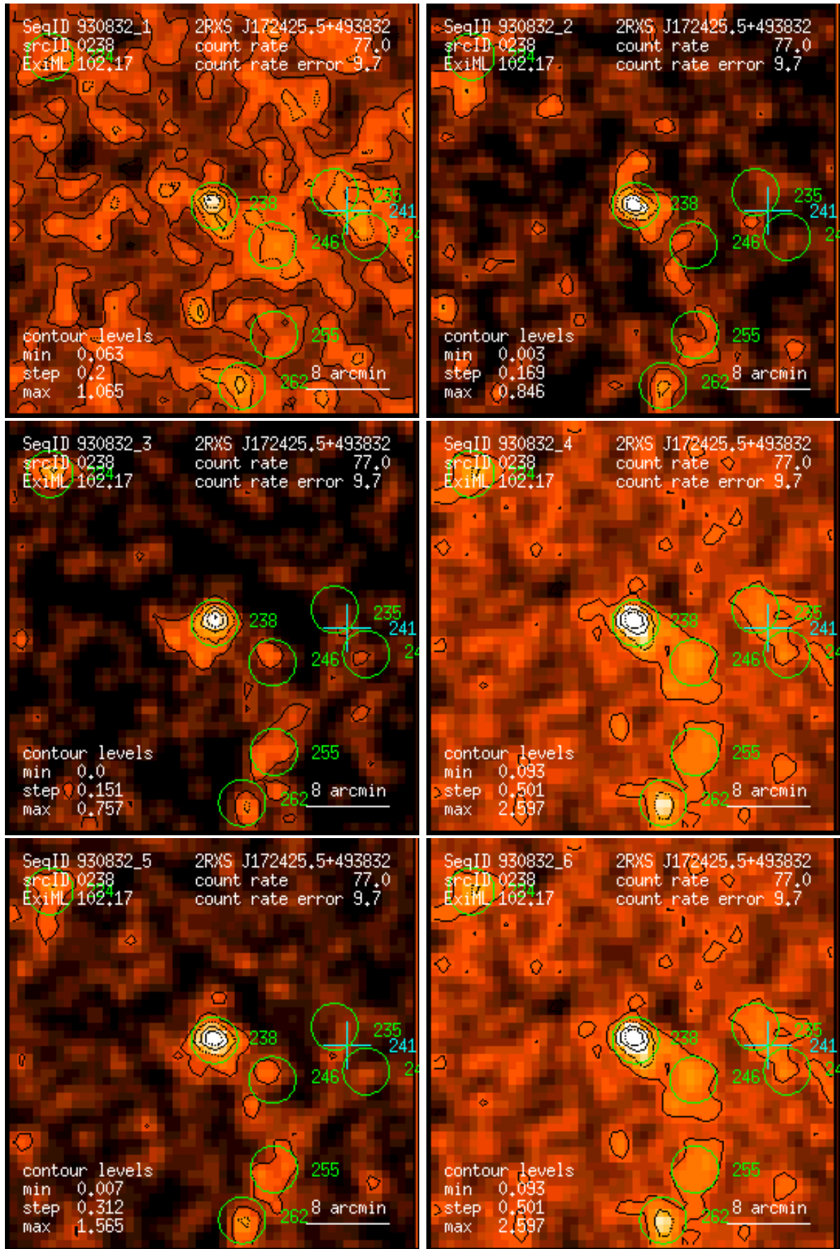
Figure 238: RASS 930832: detection 0238: band rate images, Gaussian filter: (1) PSPC channels 11 – 41, (2) 52 – 90, (3) 91 – 201, (4) 11 – 235, (5) 52 – 201, (6) 11 – 201. Broad band rates in counts/ks. Band rate contour levels in counts/ks/arcmin 2 .
