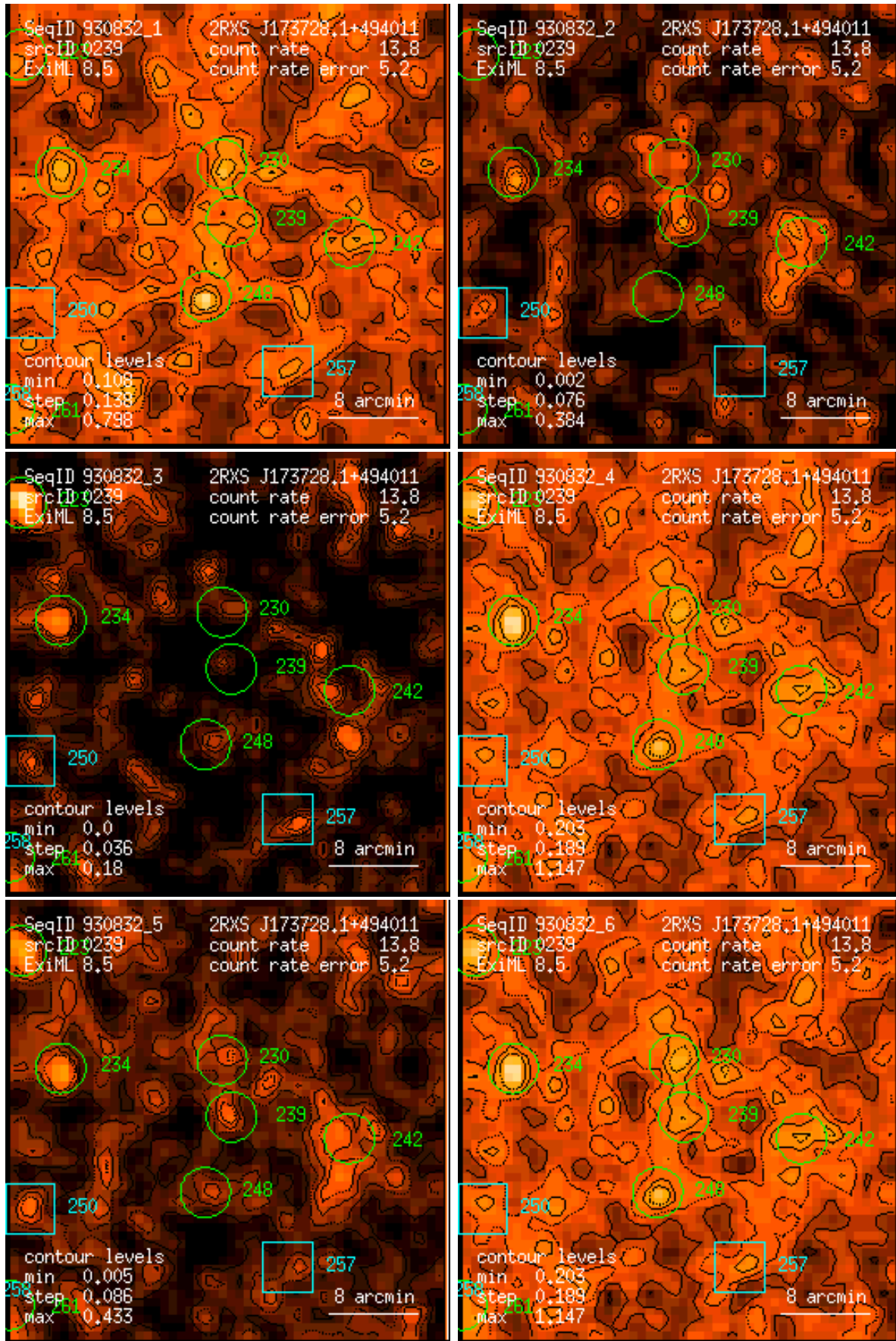
Figure 239: RASS 930832: detection 0239: band rate images, Gaussian filter: (1) PSPC channels 11 – 41, (2) 52 – 90, (3) 91 – 201, (4) 11 – 235, (5) 52 – 201, (6) 11 – 201. Broad band rates in counts/ks. Band rate contour levels in counts/ks/arcmin 2 .
