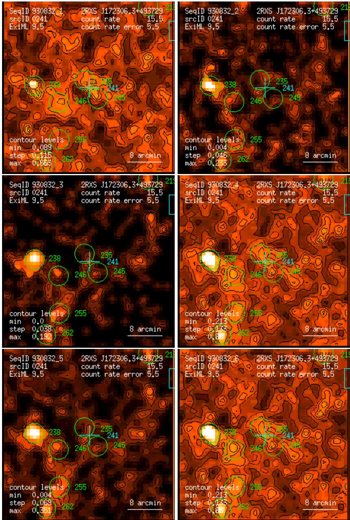
Figure 241: RASS 930832: detection 0241: band rate images, Gaussian filter: (1) PSPC channels 11 – 41, (2) 52 – 90, (3) 91 – 201, (4) 11 – 235, (5) 52 – 201, (6) 11 – 201. Broad band rates in counts/ks. Band rate contour levels in counts/ks/arcmin 2 .
